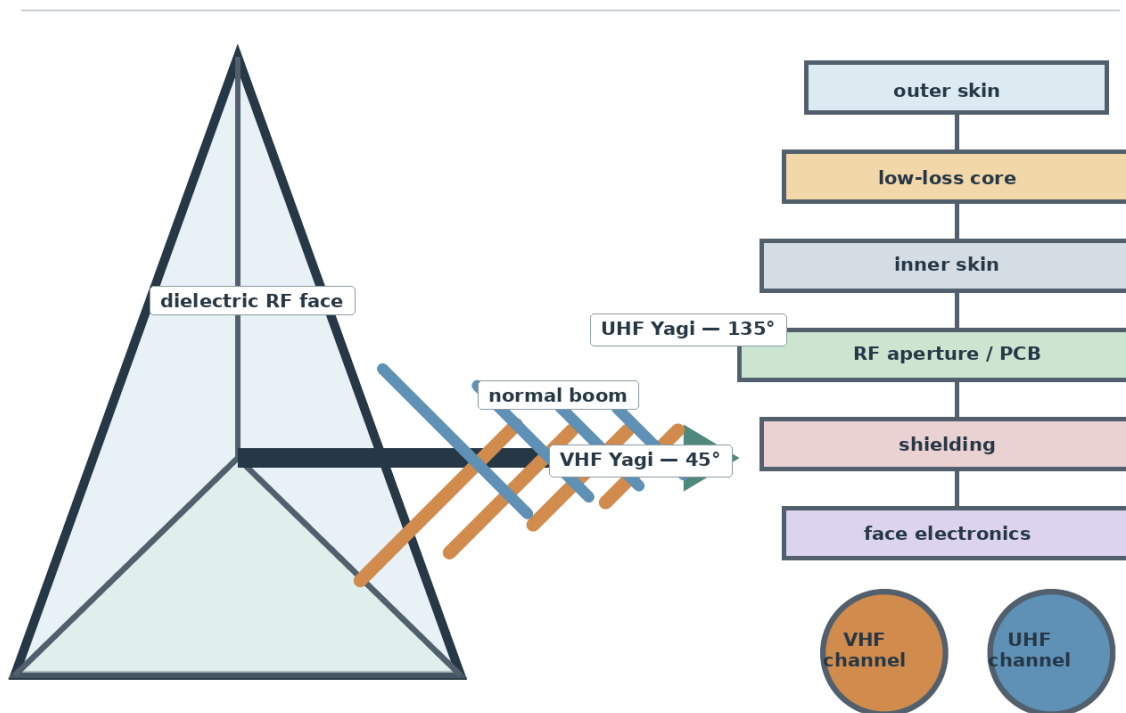
Figure 3.2: Face assembly. The dark boom follows the outward normal from the inward apex through the centre of the two-metre triangular aperture; orange and blue elements are mutually orthogonal and jointly rotated 45° around that normal. The coloured plates at right represent the material and electronics stack.
