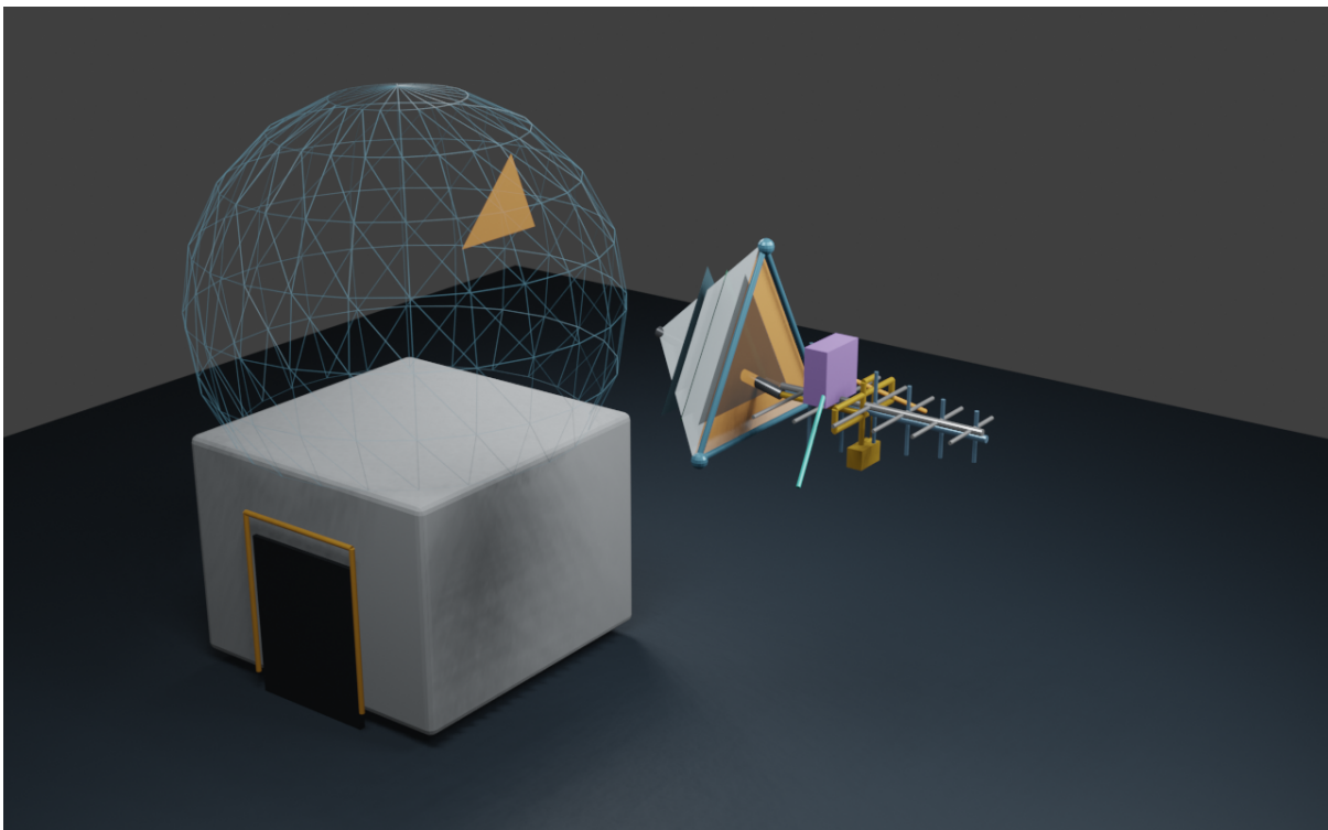
Figure 3.7: Blender Eevee render of the radome and exploded face. The external VHF and UHF Yagis share the support/boom axis and use orthogonal transverse elements.
