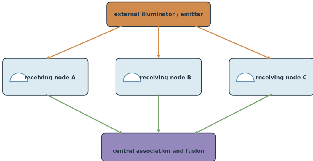
Figure 2.1: Distributed sensing architecture: the upper polygon is an illuminator or emitter, the three domes are independent receiving nodes, green paths carry calibrated observations, and the lower purple block is central fusion.
