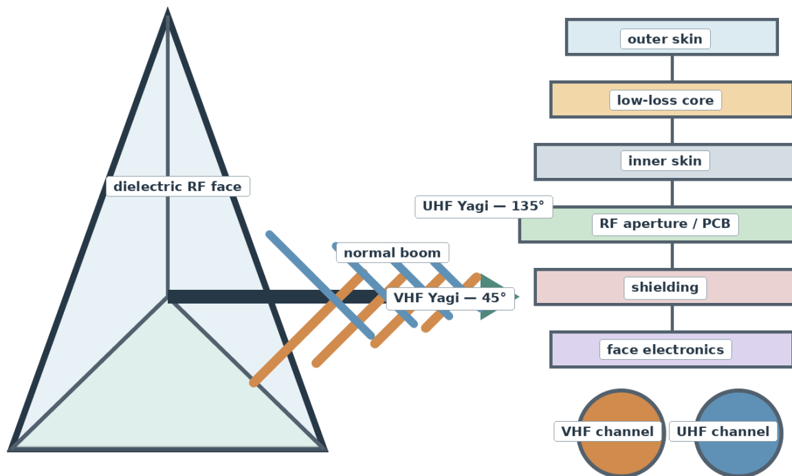
Figure 3.2: Face assembly. The dark boom follows the outward normal from the inward apex through the centre of the two-metre triangular aperture; orange and blue elements are mutually orthogonal and jointly rotated 45° around that normal. The coloured plates at right represent the material and electronics stack.
