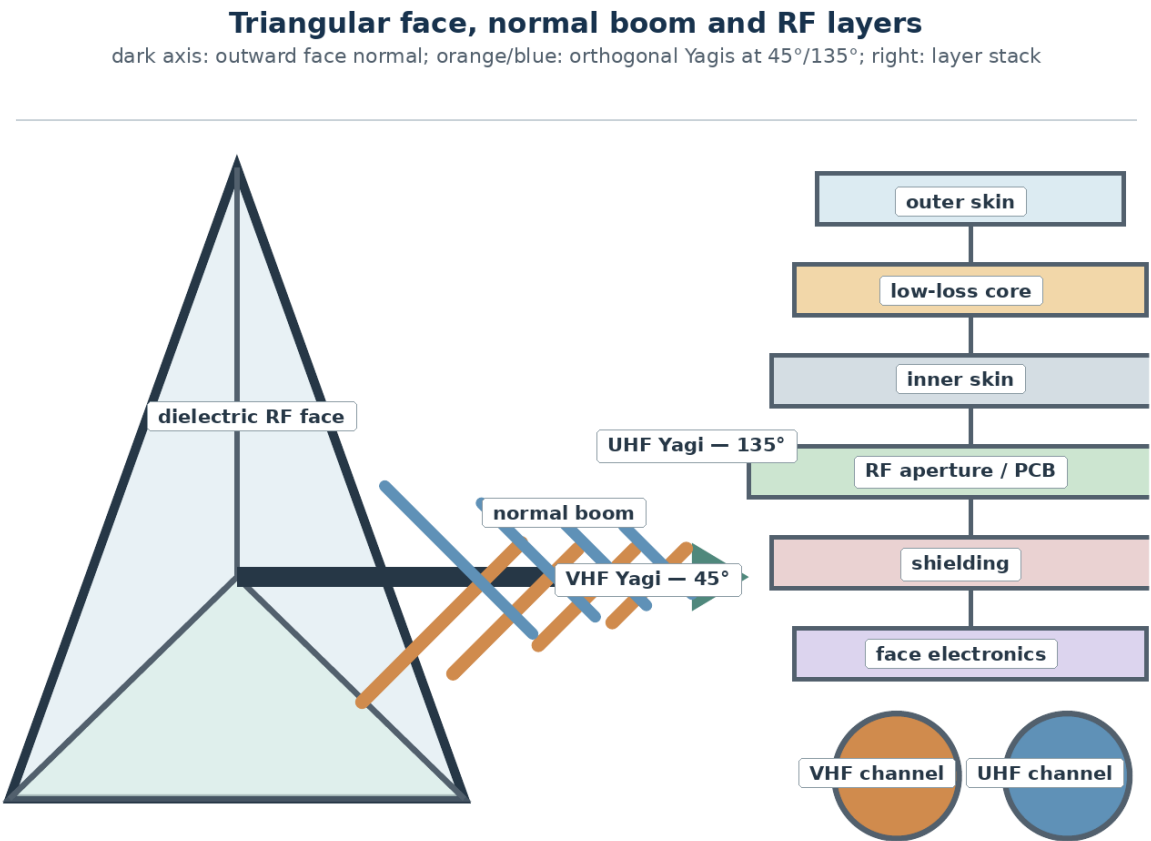
Figure 3.2: Face assembly. The dark boom follows the outward normal from the inward apex through the centre of the two-metre triangular aperture; orange and blue elements are mutually orthogonal and jointly rotated 45° around that normal. The coloured plates at right represent the material and electronics stack.
