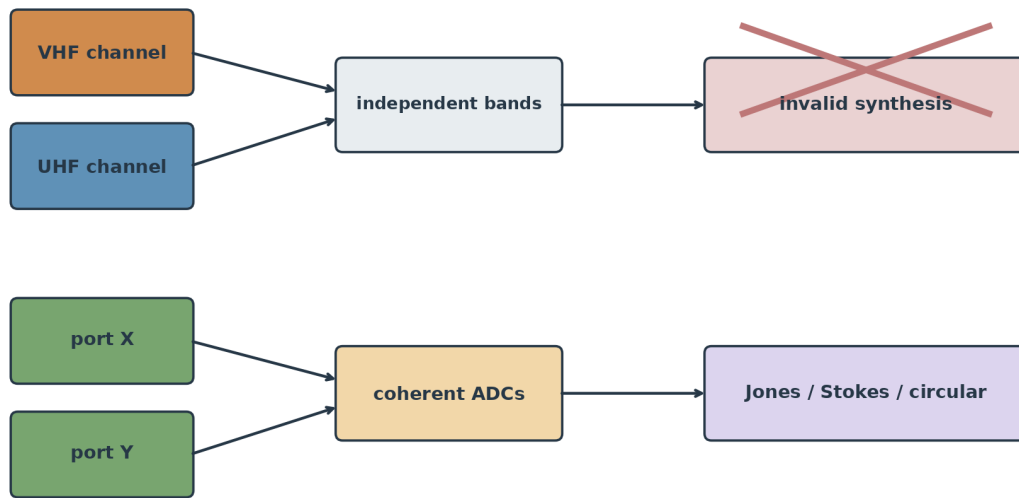
Figure 4.2: Top flow: independently digitized VHF and UHF channels terminate in a crossed-out cross-band polarimetric result. Bottom flow: two coherent orthogonal ports in the same band feed calibrated Jones, Stokes or circular-polarization products.
