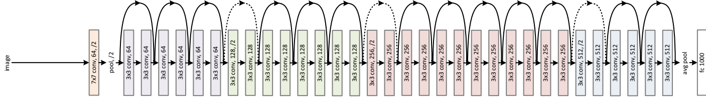
34-layer residual
