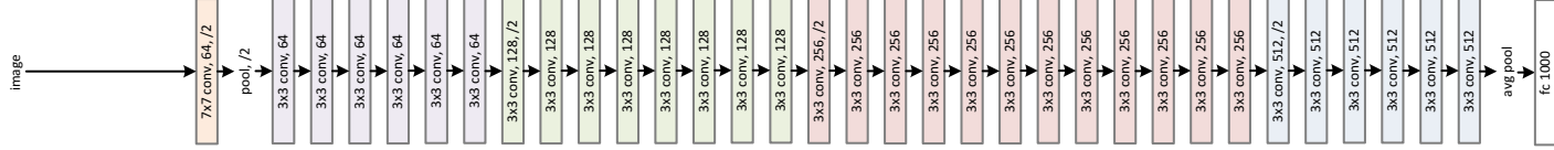
34-layer plain
