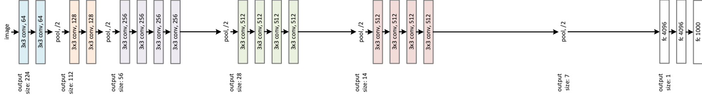
VGG-19
