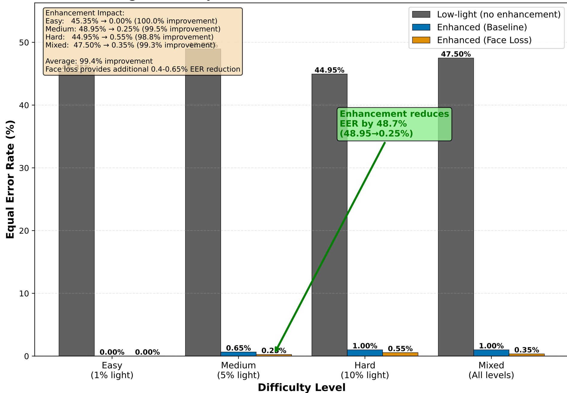
Figure 10: Impact of Enhancement on Face Verification
