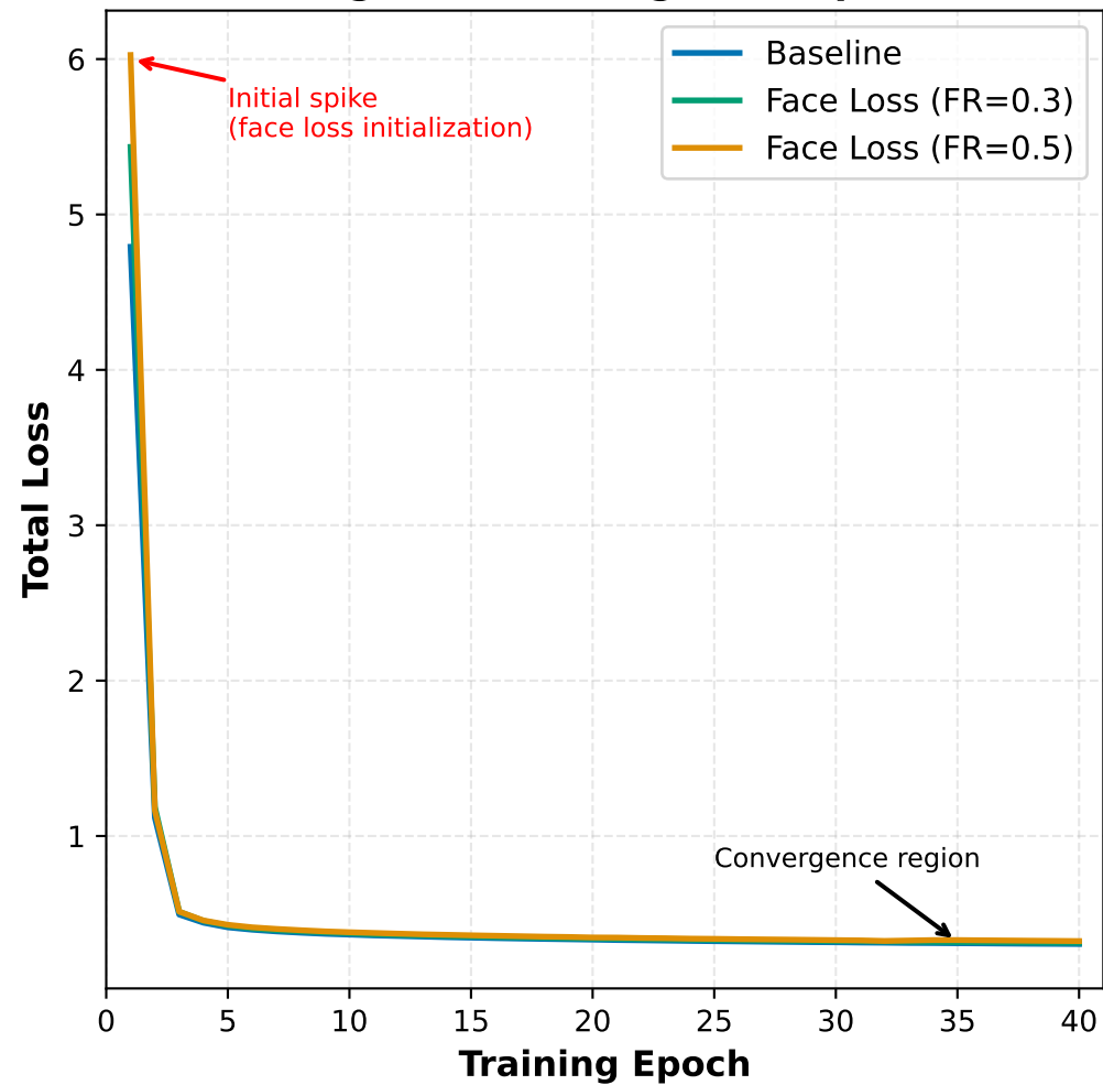
(A) Training Loss Convergence (Epochs 1-40)
