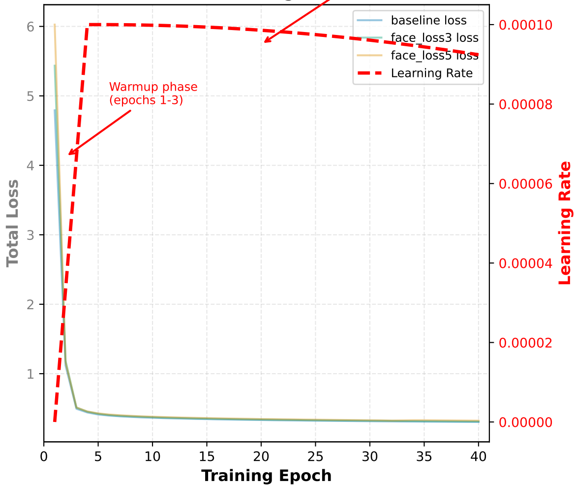
(B) Loss vs. Learning Rate Schedule
