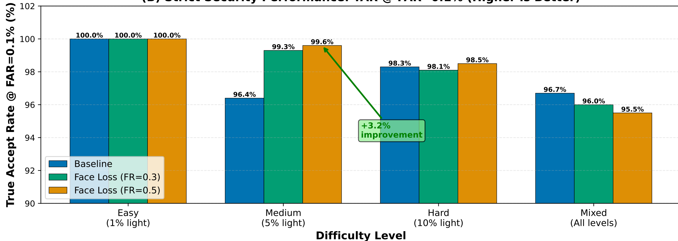
(B) Strict Security Performance: TAR @ FAR=0.1% (Higher is Better)
