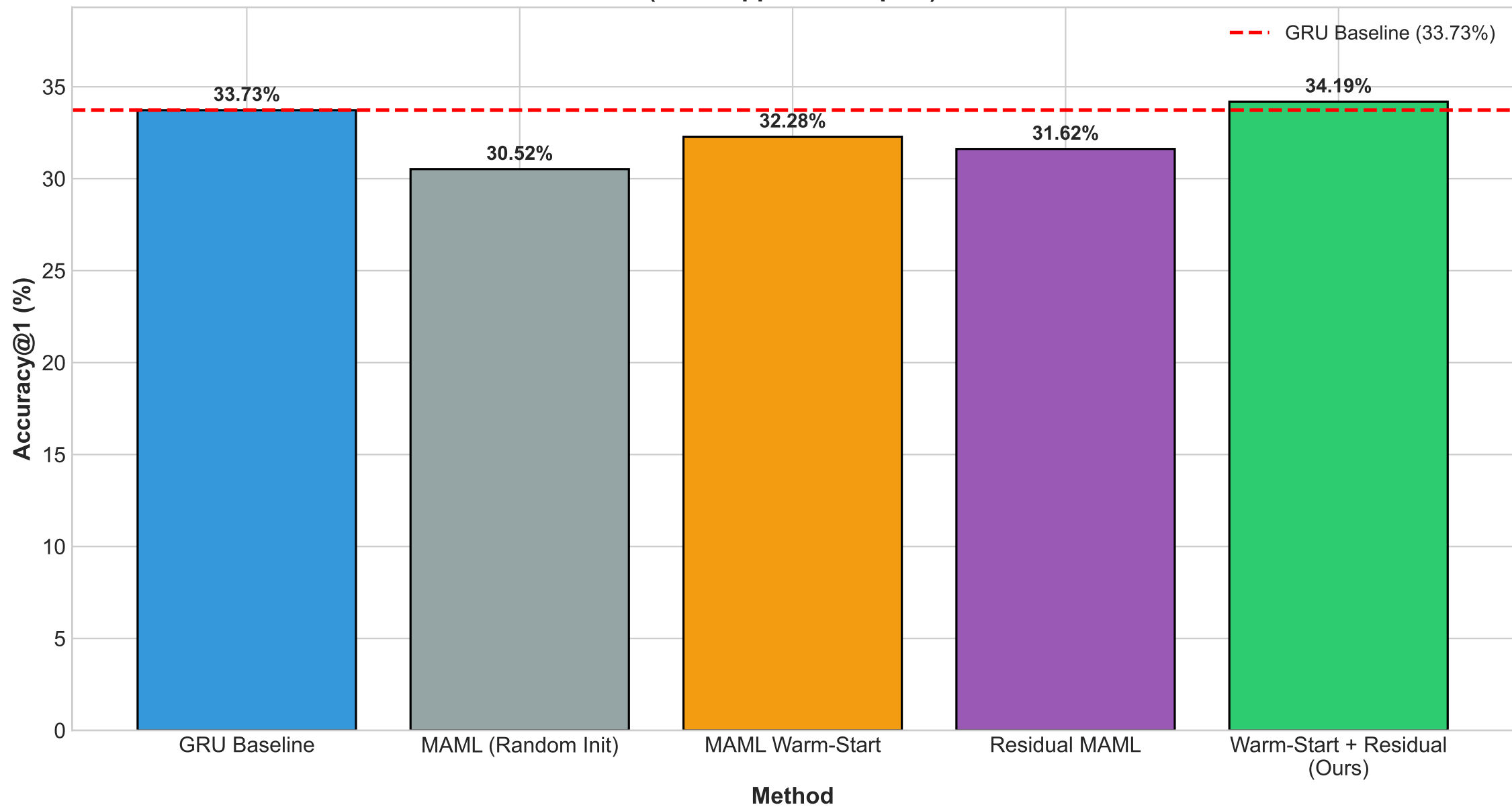
Cold-Start Recommendation Performance on XuetangX (K=5 Support Examples)
