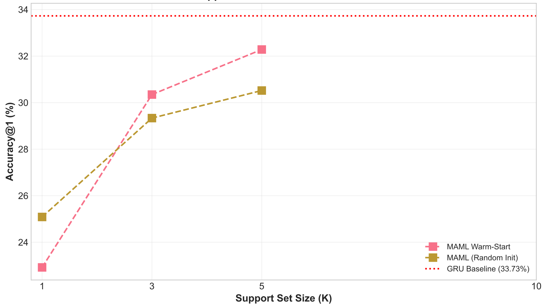
Effect of Support Set Size on Cold-Start Performance
