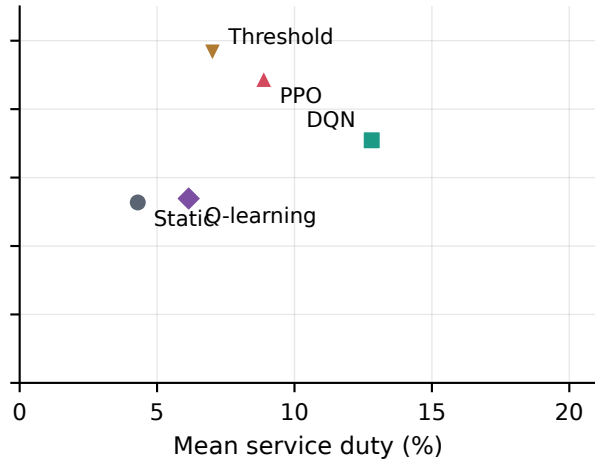
Process runtime
