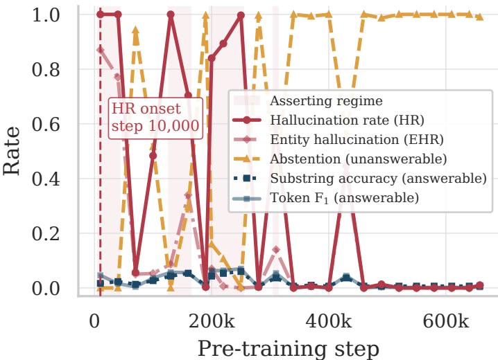
(a) Recall and fabrication along training
