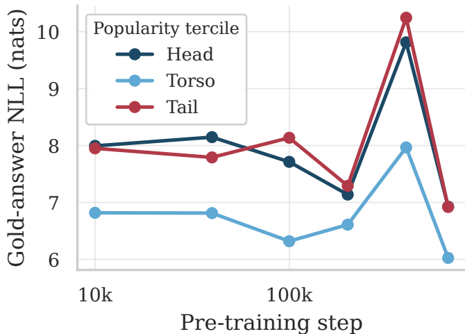
(b) Gold-answer likelihood
