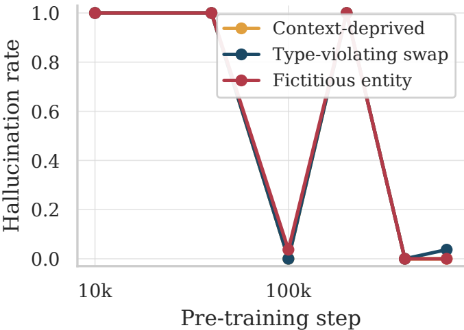
(a) Fabrication by unanswerability type
