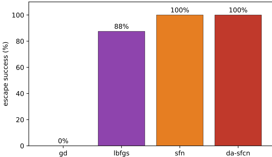
Saddle escape (8 seeds, n=40)
