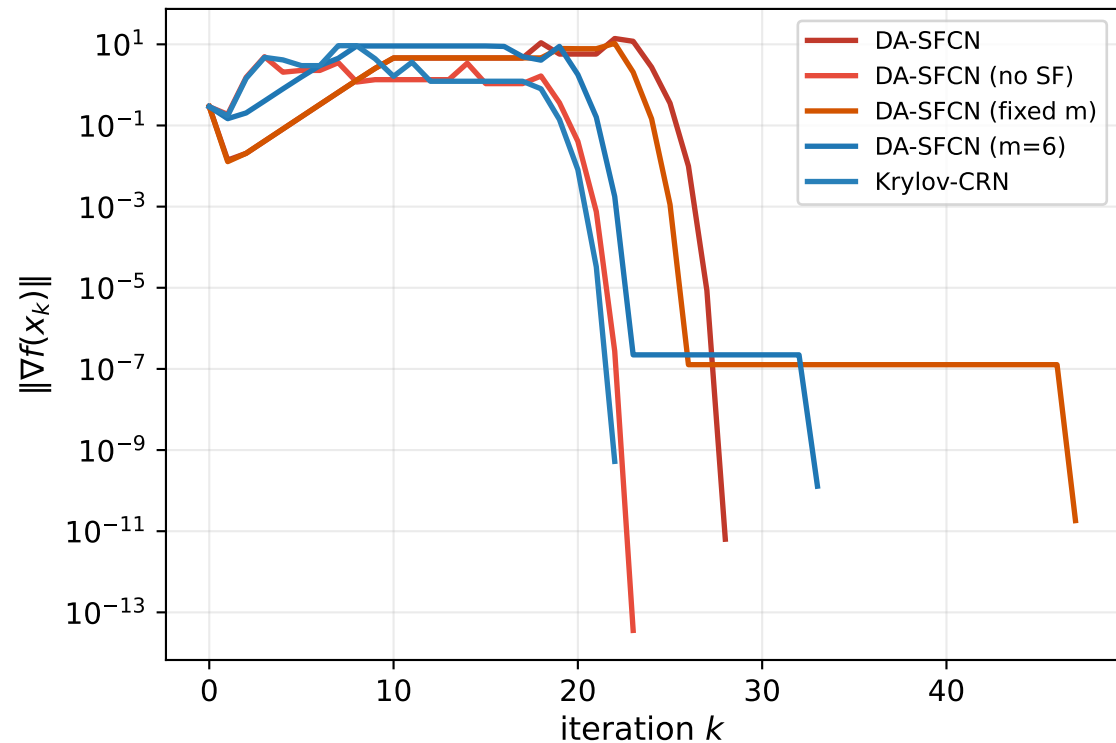
Ablation: saddle-free and dynamic m_k
