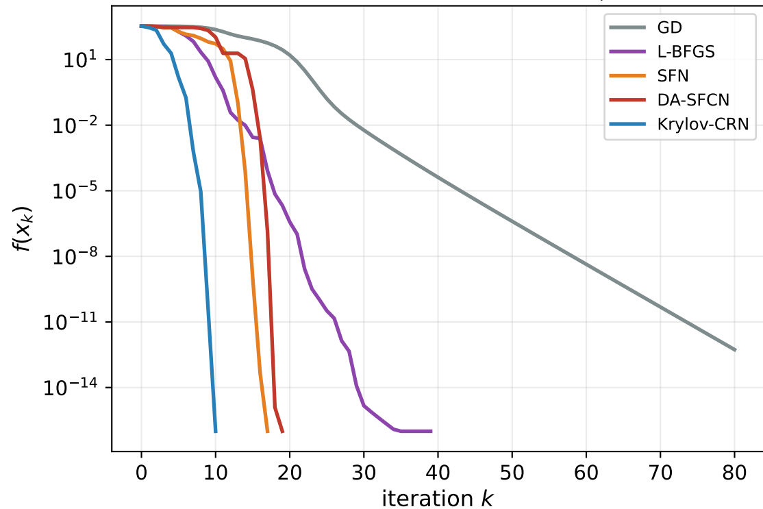
Matrix factorization \|X - UV^\top\|_F^2
