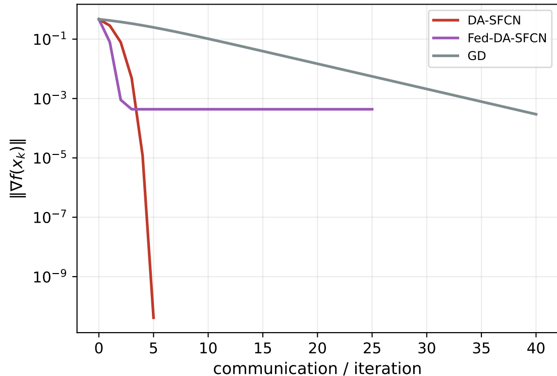
Federated nonconvex logistic
