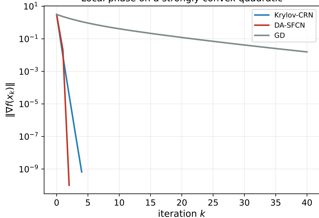
Local phase on a strongly convex quadratic
