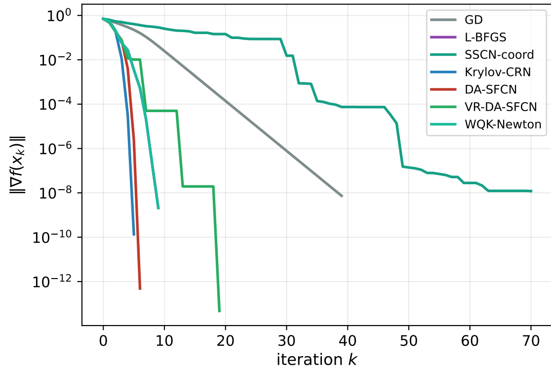
Nonconvex logistic regression
