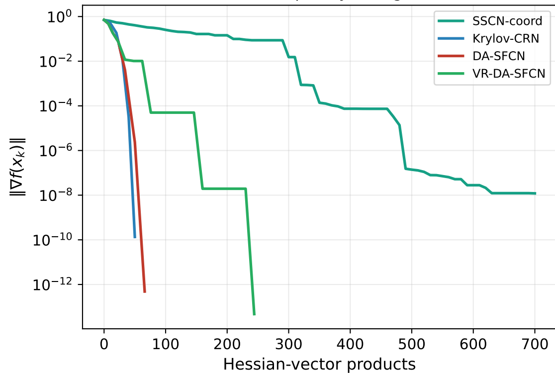
Oracle complexity on logistic
