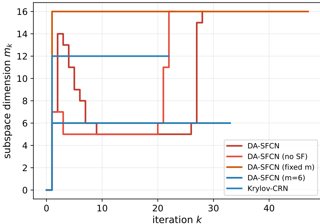
Dynamic Krylov dimension
