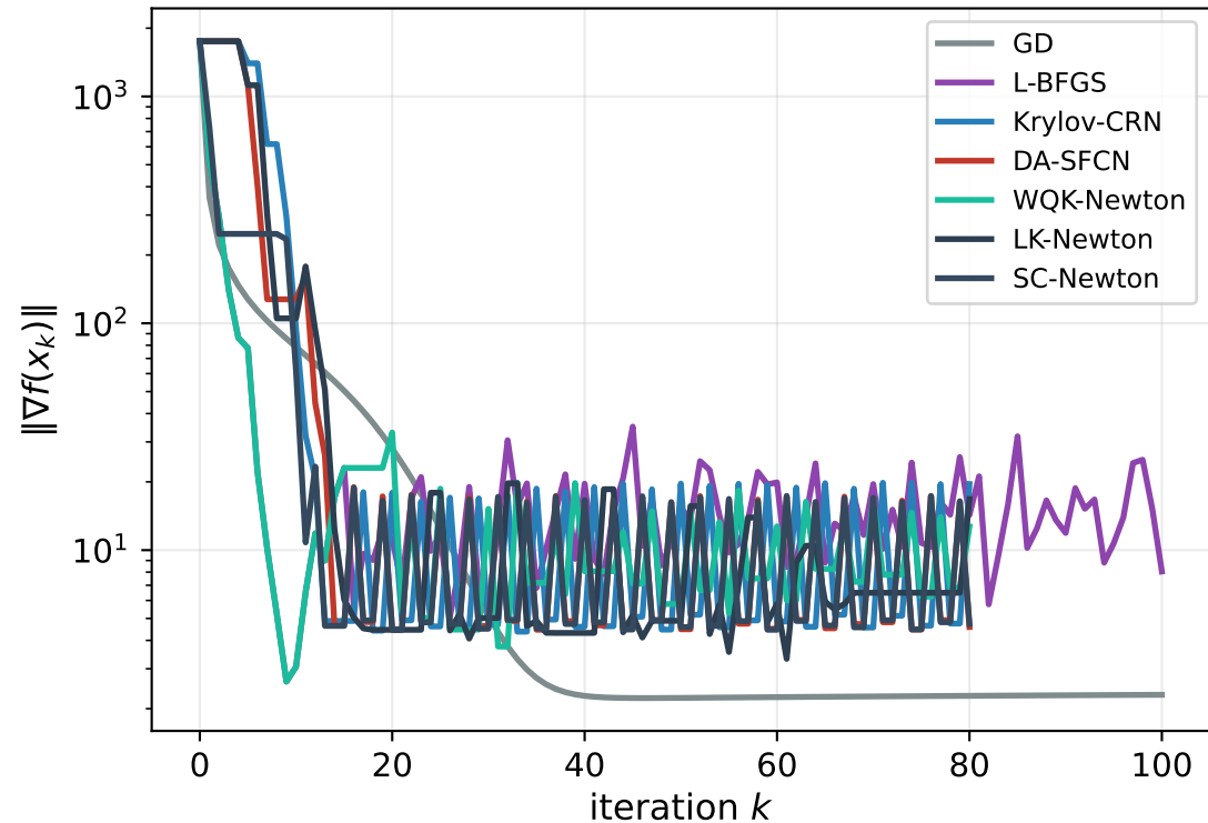
Extended Rosenbrock ( n = 40 )
