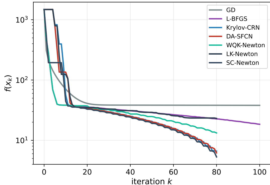
Rosenbrock objective
