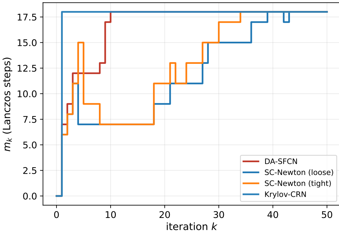
Work per iteration under the spectral certificate
