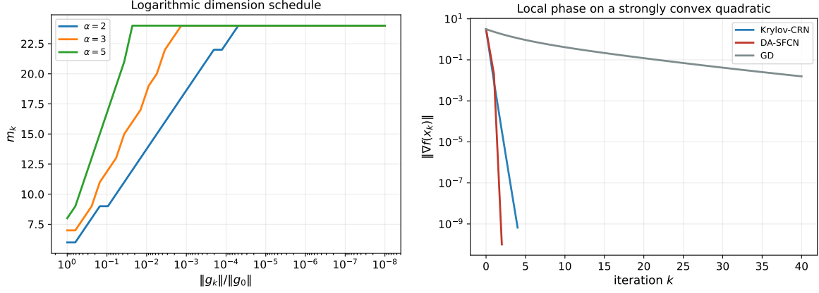
Figure 3: Logarithmic m_k and the local Newton phase.
