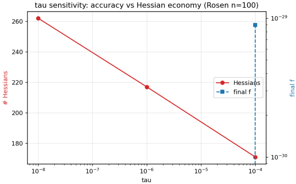
Figure 4: Accuracy vs Hessian economy trade-off as a function of \tau .
