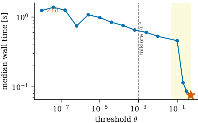
quadratic \kappa = 10^3 , n = 1000
