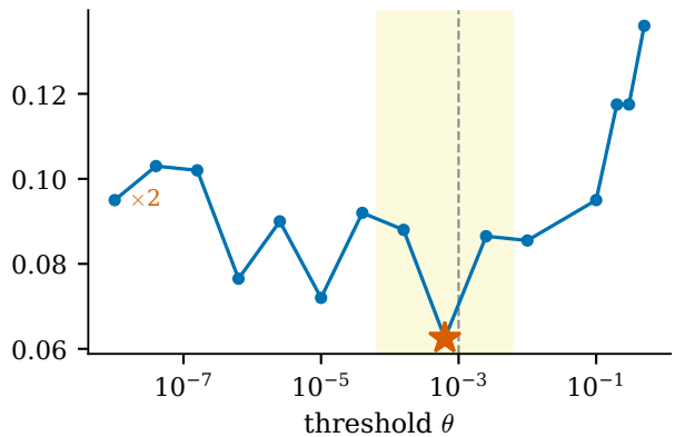
logistic \lambda = 0.01 , m = 200 , n = 200
