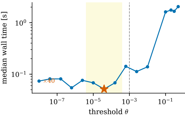
log-sum-exp m = 300 , n = 50
