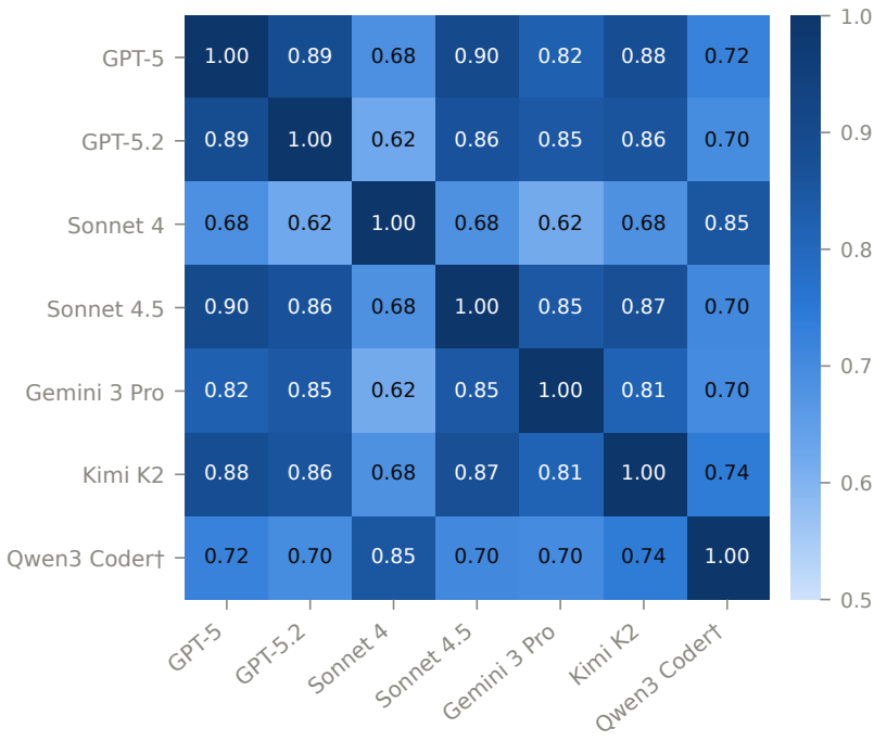
Outcome correlation across 275 tasks
