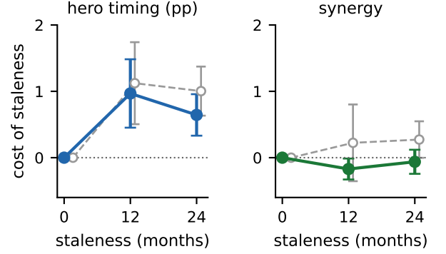
Fig. 2. Cost of staleness in future-meta hero win rate (left, pp) and synergy (right), scored on out-of-sample builds, with 95% t intervals from crossed seed random effects. The agent trained at the 2026 cutoff (0 months, the reference) against leak-free agents trained one and two years earlier. Filled: opponent models matched by era on both sides (U-era against S1, S2). Hollow: the 2026 agent on the earlier paper’s opponent model, which saw the test period (U against S1, S2).
