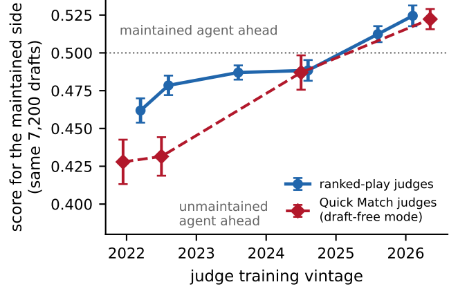
Fig. 4. The vintage matrix. Score assigned to the maintained side of the 7,200 leak-free MAINTAINED versus UNMAINTAINED drafts by win-probability judges trained at different times (95% intervals, normal approximation, clustered by seed pairing; judge-seed variation is not included). Realized outcomes favor the maintained side. Judges trained before 2023 reverse the verdict, and judges from 2025 on agree with it. Diamonds: judges trained on Quick Match, a mode without a draft phase.
