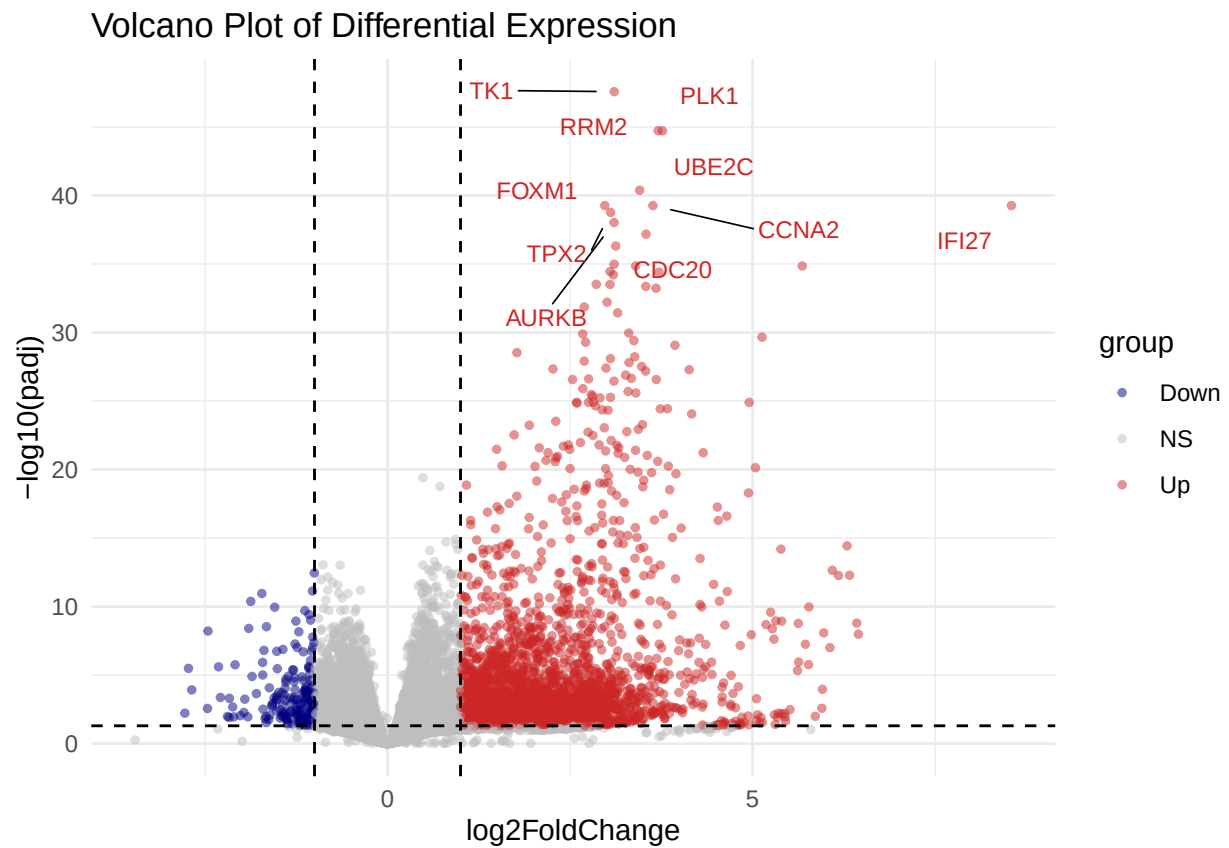
Figure 2: Volcano plot of differential gene expression showing \log_2 fold change versus statistical significance. Thresholds of |\log_2\text{FC}| > 1 and adjusted p-value < 0.05 are indicated by dashed lines. Red points represent upregulated genes, blue points represent downregulated genes, and grey points are not significant.
