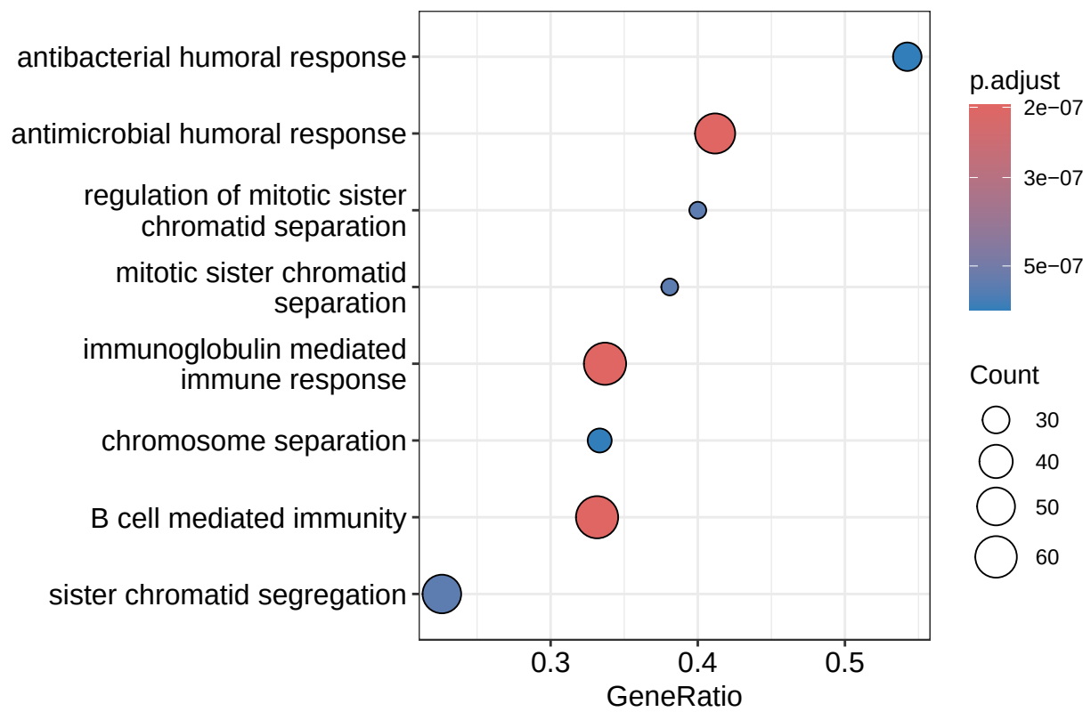
Figure 6: Gene Set Enrichment Analysis (GSEA) dotplot showing significant enrichment of immune-related and cell cycle-associated biological processes.
