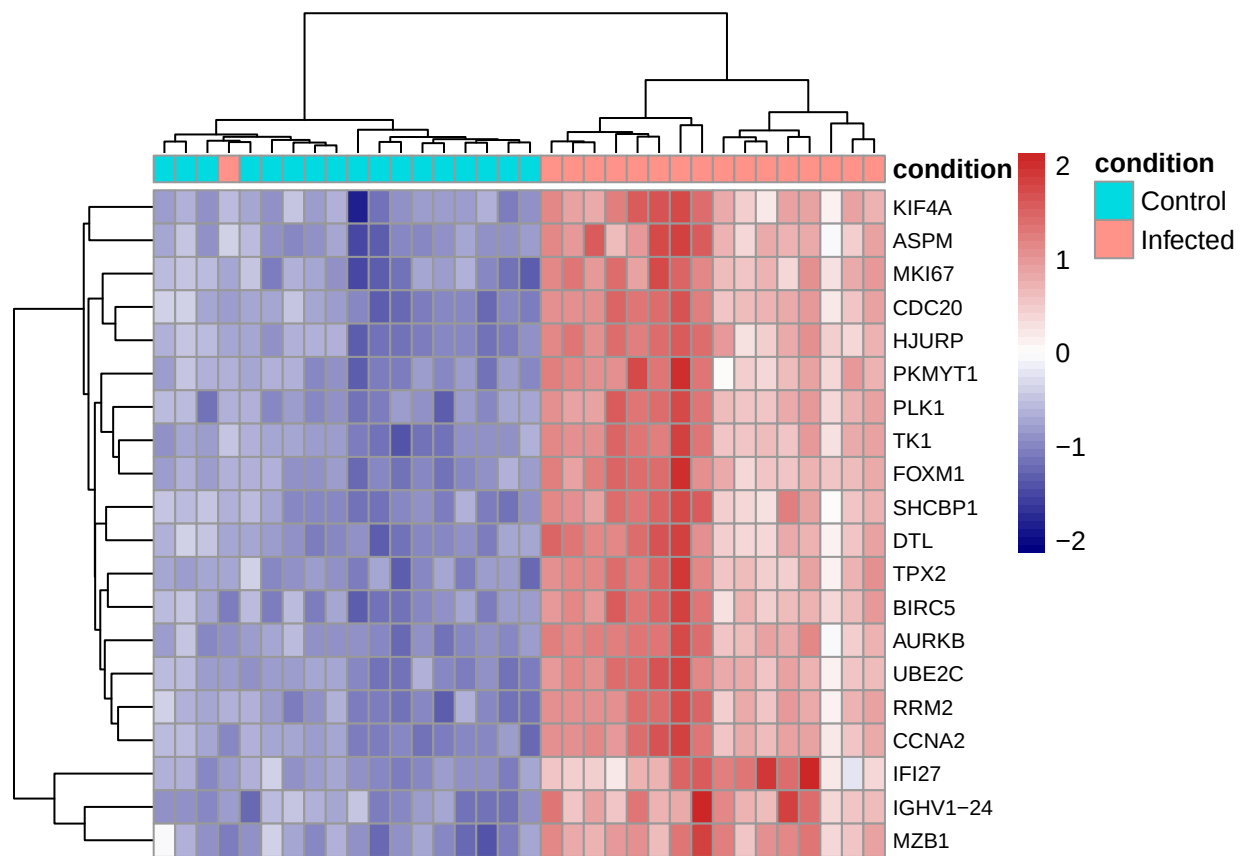
Figure 4: Heatmap of the top 20 differentially expressed genes showing distinct clustering of infected and control samples, indicating consistent expression patterns within each condition.
