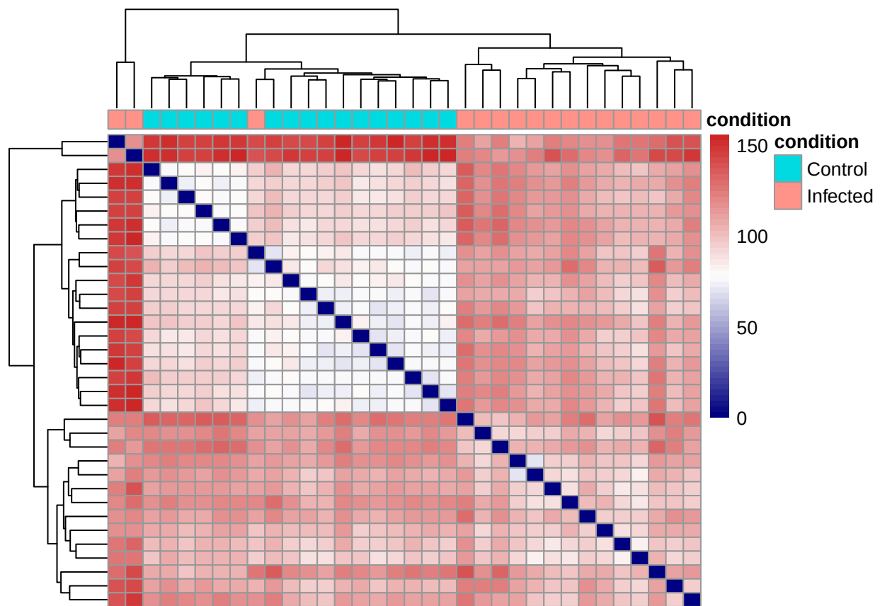
Figure 5: Sample-to-sample distance heatmap demonstrating clustering based on global gene expression profiles, with infected samples grouping separately from controls.
