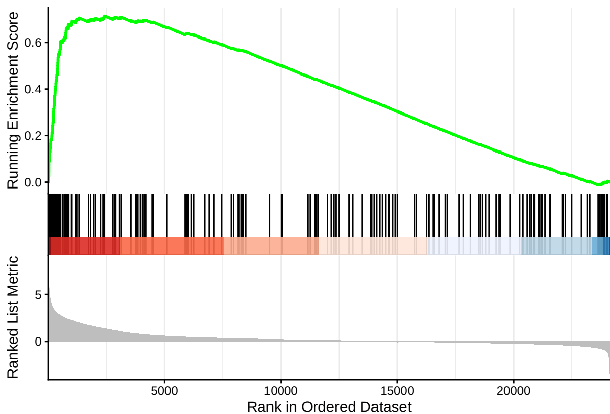
Figure 7: GSEA enrichment plot for the top enriched pathway, illustrating the distribution of pathway-associated genes across the ranked gene list and their contribution to the enrichment score.
