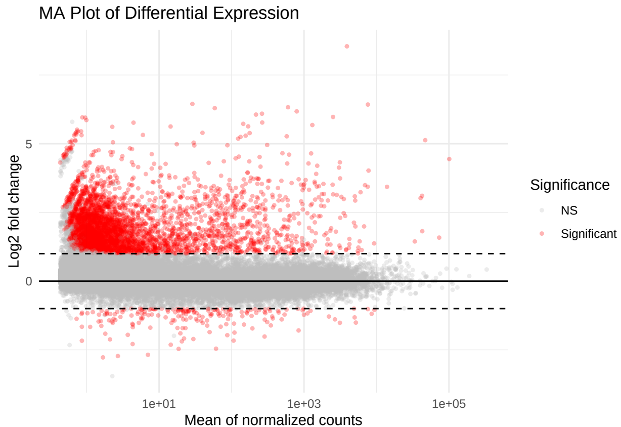
Figure 3: MA plot showing the relationship between mean expression and log2 fold change, demonstrating that differential expression occurs across a wide range of expression levels.
