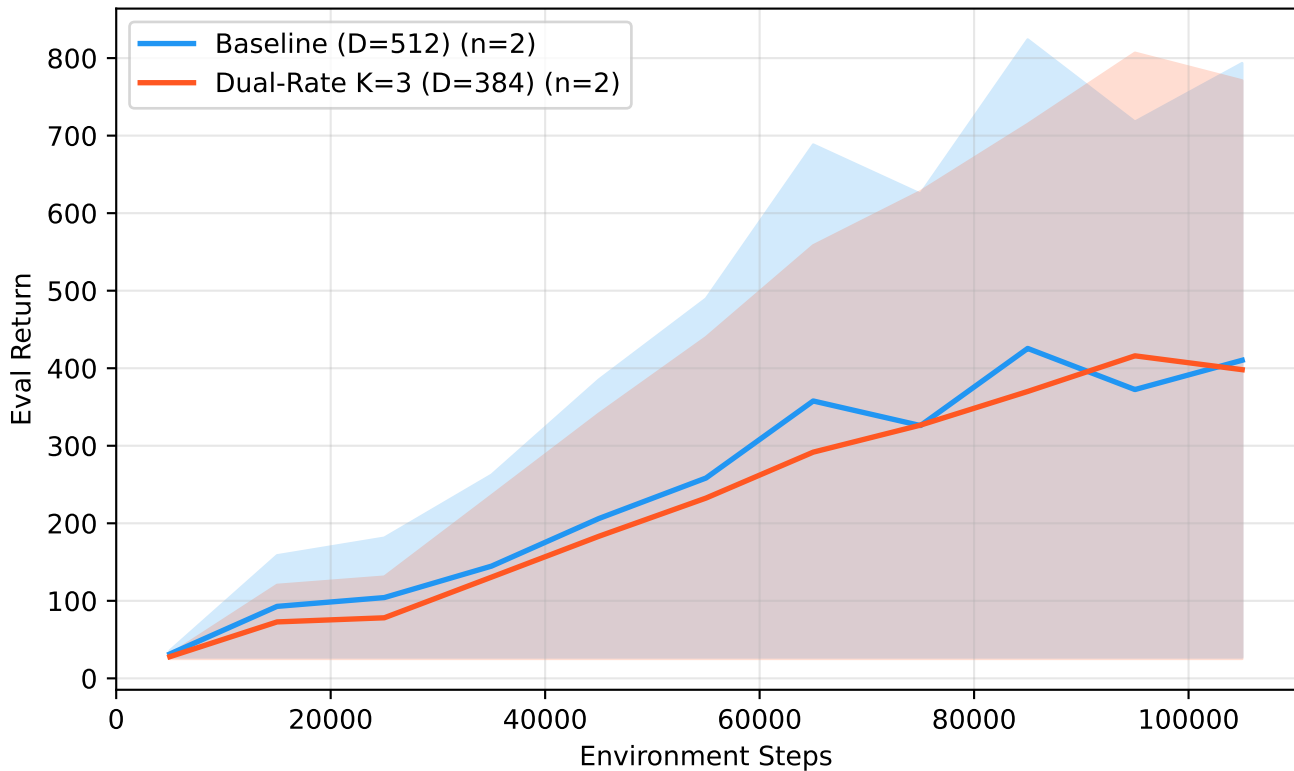
DMControl Walker-Walk: Eval Return
