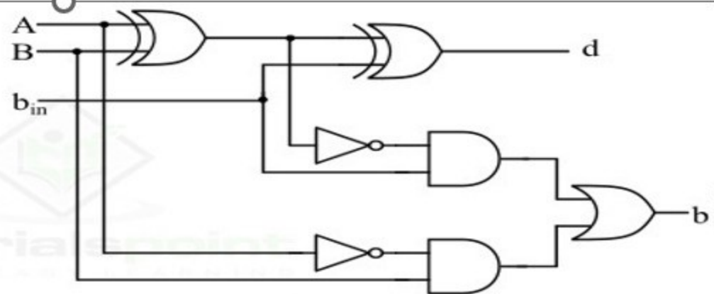
Figure 1 - Full Subtractor
