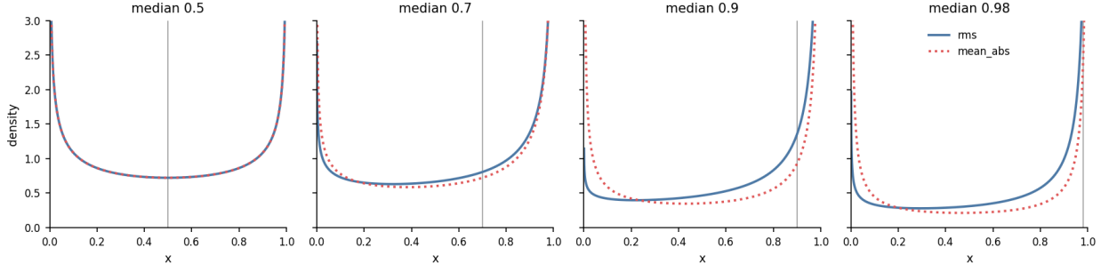
Figure 1: Density of one coordinate of a pixel's voters, D = 0.3 , for medians moving towards the wall at 1 (grey: the median). Both rules agree at the centre. Near the wall mean_abs moves many voters to the opposite wall; rms moves far fewer.
