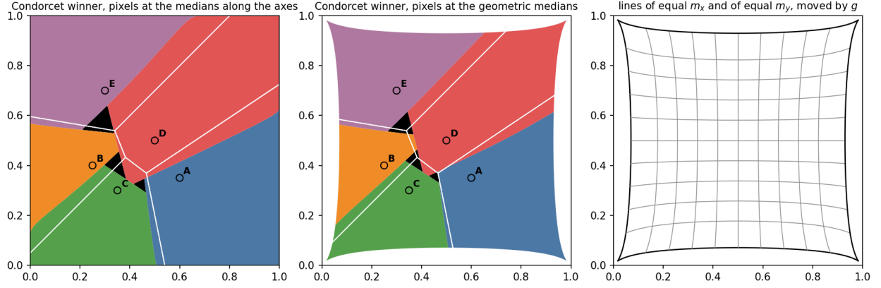
Figure 16: Beta voters ( rms , D = 0.3 ). Left and middle: the Condorcet winner with pixels at the medians along the axes and at the geometric medians. White lines: the Voronoi borders (bisectors); black: no Condorcet winner. Right: the lines of equal m_x and of equal m_y , moved by g ; the thick outline belongs to the outermost medians.
