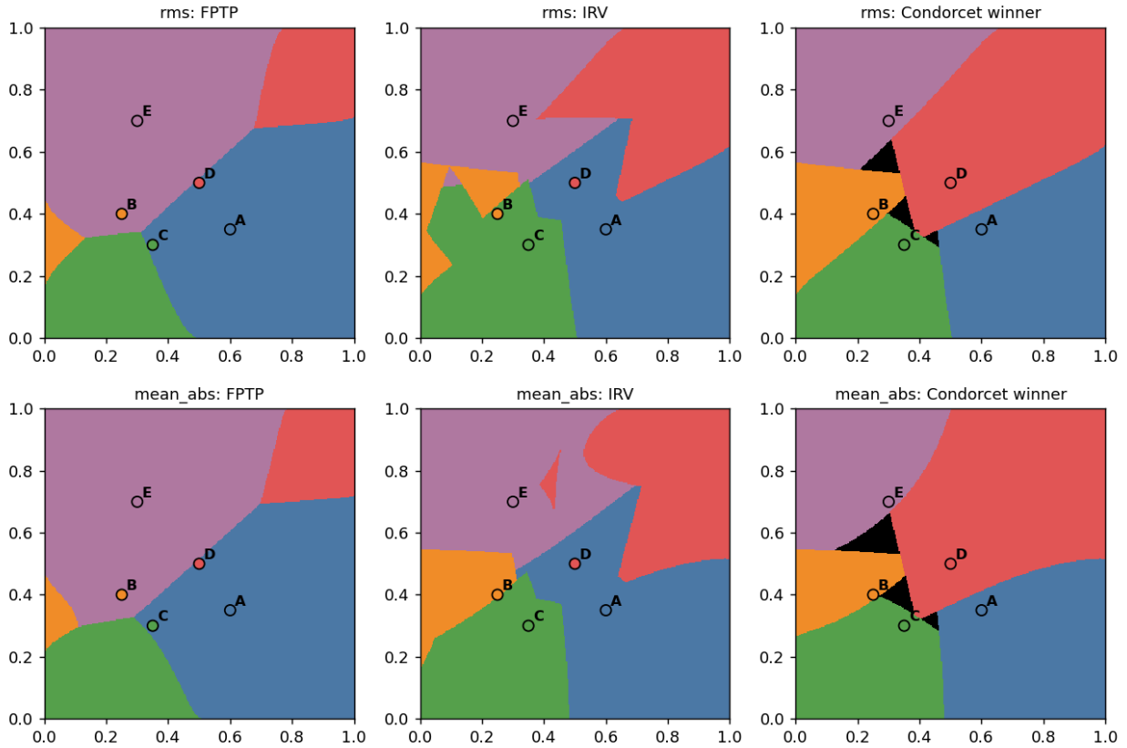
Figure 9: The two spread rules of Section 1.5 on the default candidates, D = 0.3 . Only mean_abs has the round IRV edge. Black: no Condorcet winner.
