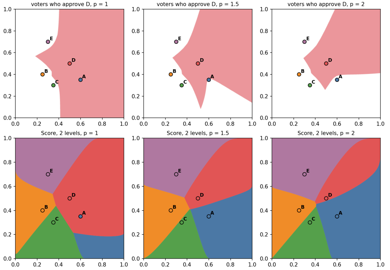
Figure 3: Two levels at the ends and the default of the slider, p = 1, 1.5 and 2 . Top: the voters who approve D, those beyond 2^{-1/p} of the way from the farthest candidate to the closest; the borders are curves. Bottom: the diagrams (candidates A–E, Beta voters, rms, D = 0.2 ).
