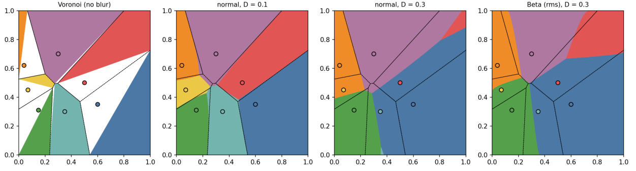
Figure 7: FPTP for seven candidates; dashed: Voronoi borders. From left: no blur (Voronoi), normal voters with D = 0.1 and D = 0.3 , Beta voters (rms) with D = 0.3 .
