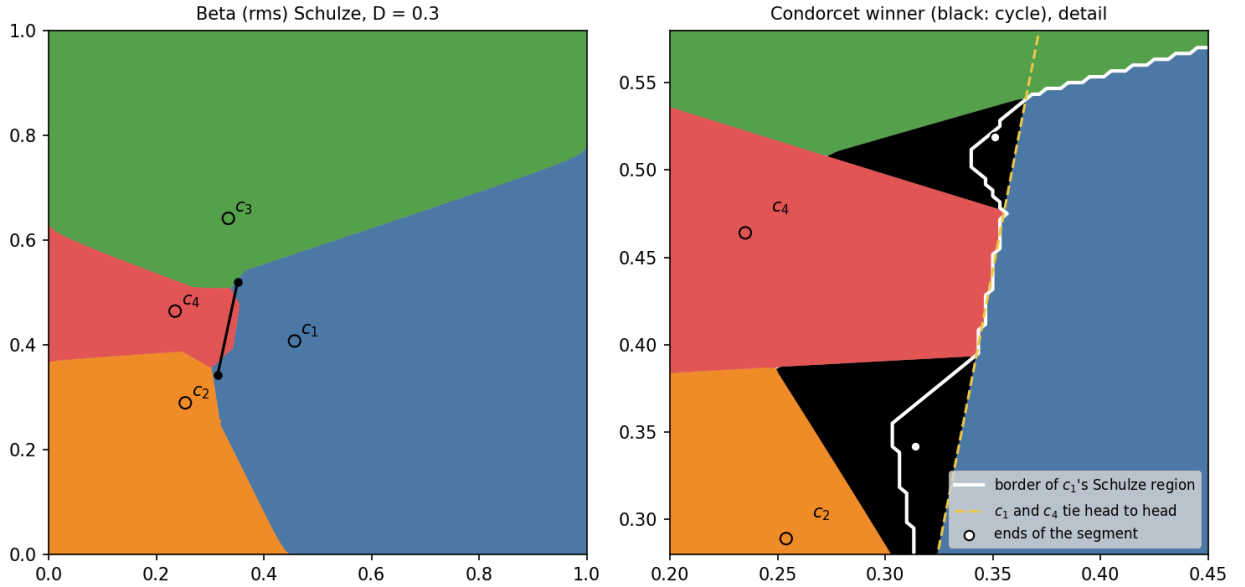
Figure 13: Left: Schulze with Beta voters (rms, D = 0.3 ). c_1 (blue) wins at both ends of the segment, c_4 (red) in between. Right: detail with the Condorcet winner (black: cycles). c_1 's Schulze region, to the right of the white line, reaches across the tie line of c_1 and c_4 (yellow) into two cycle pockets.
