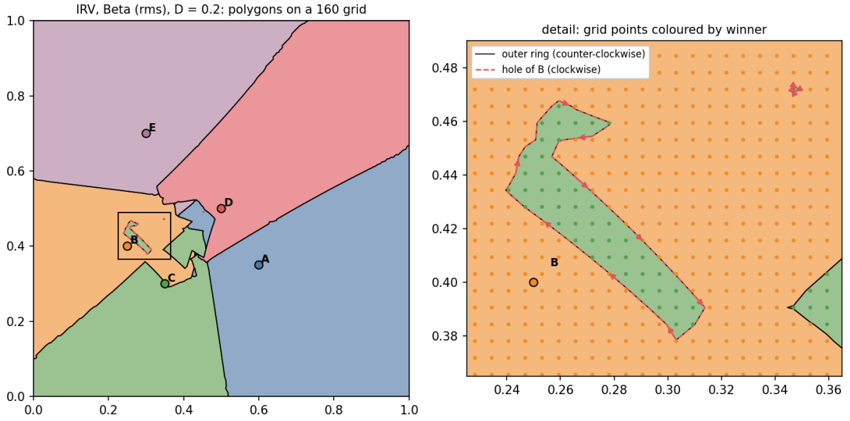
Figure 16: The polygons of Table 10, filled with the even-odd rule as in the UI. Solid black: outer rings; dashed red: holes. Right: the frame on the left, with the grid points coloured by their winner. The arrows run clockwise along B’s two holes: the island of C, and at the top right a sliver of C that the grid catches at only one point.
