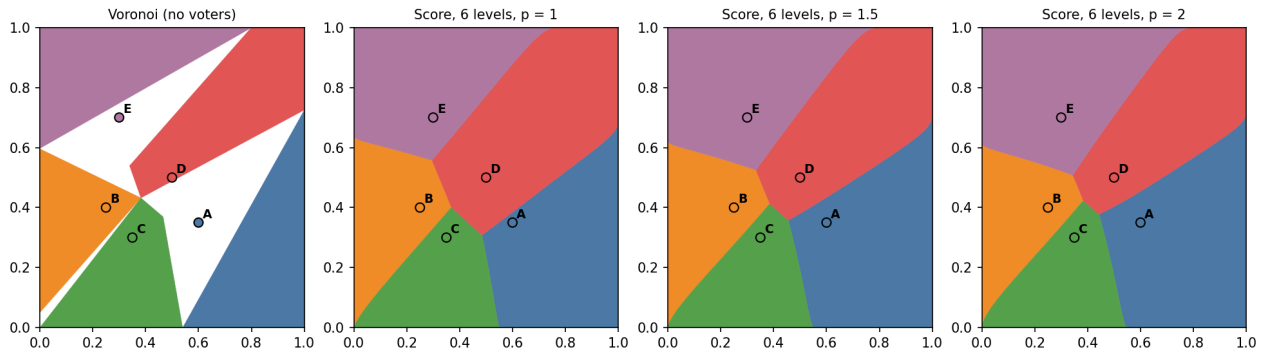
Figure 4: Six levels, the default, at p = 1, 1.5 and 2 , next to the Voronoi diagram (candidates A–E, Beta voters, rms, D = 0.2 ).
