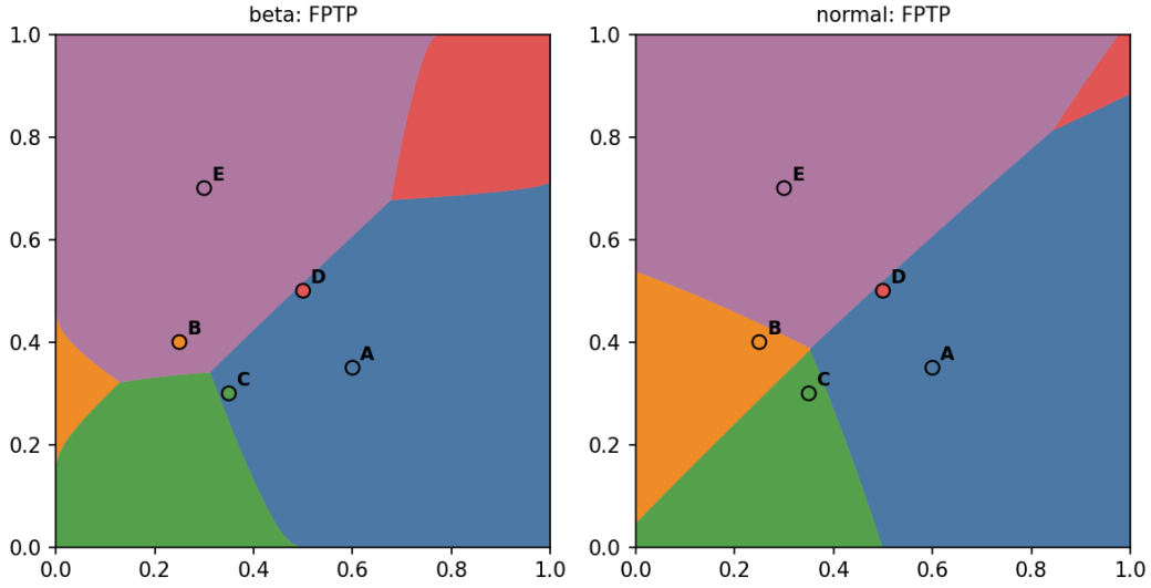
Figure 8: FPTP. With Beta voters the region of B flares out in the last few hundredths before the left wall; with normal voters it widens smoothly.
