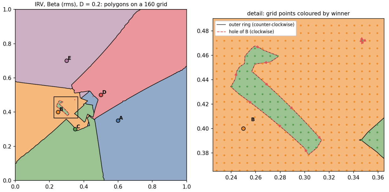
Figure 14: The polygons of Table 4, filled with the even-odd rule as in the UI. Solid black: outer rings; dashed red: holes. Right: the frame on the left, with the grid points coloured by their winner. The arrows run clockwise along B's two holes: the island of C, and at the top right a sliver of C that the grid catches at only one point.
