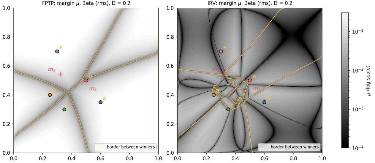
Figure 13: The margin \mu of FPTP (left) and IRV (right) on the grid of G = 320 points per axis (Beta, rms, D = 0.2 ), on a log scale: black is below 10^{-4} . Yellow: the borders between winners, traced as in Section 7.5.2. The crosses mark m_1 (at D) and m_2 .
