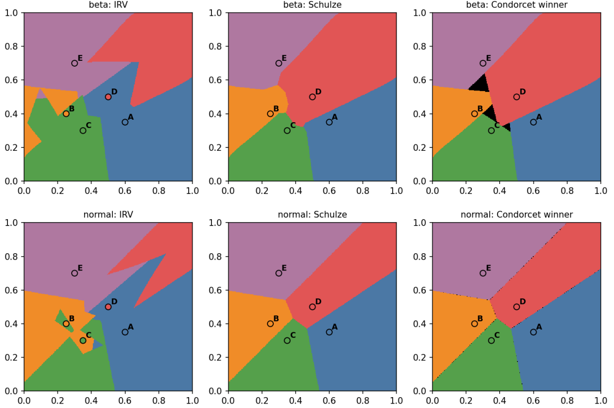
Figure 3: Beta voters (rms, top) and normal voters (bottom), D = 0.3 . Normal Schulze and the normal Condorcet winner are exactly the Voronoi diagram of the candidates. Black: no Condorcet winner. The dotted black lines in the bottom right plot are pixels whose centre lies exactly on a bisector (a tie, not a cycle).
