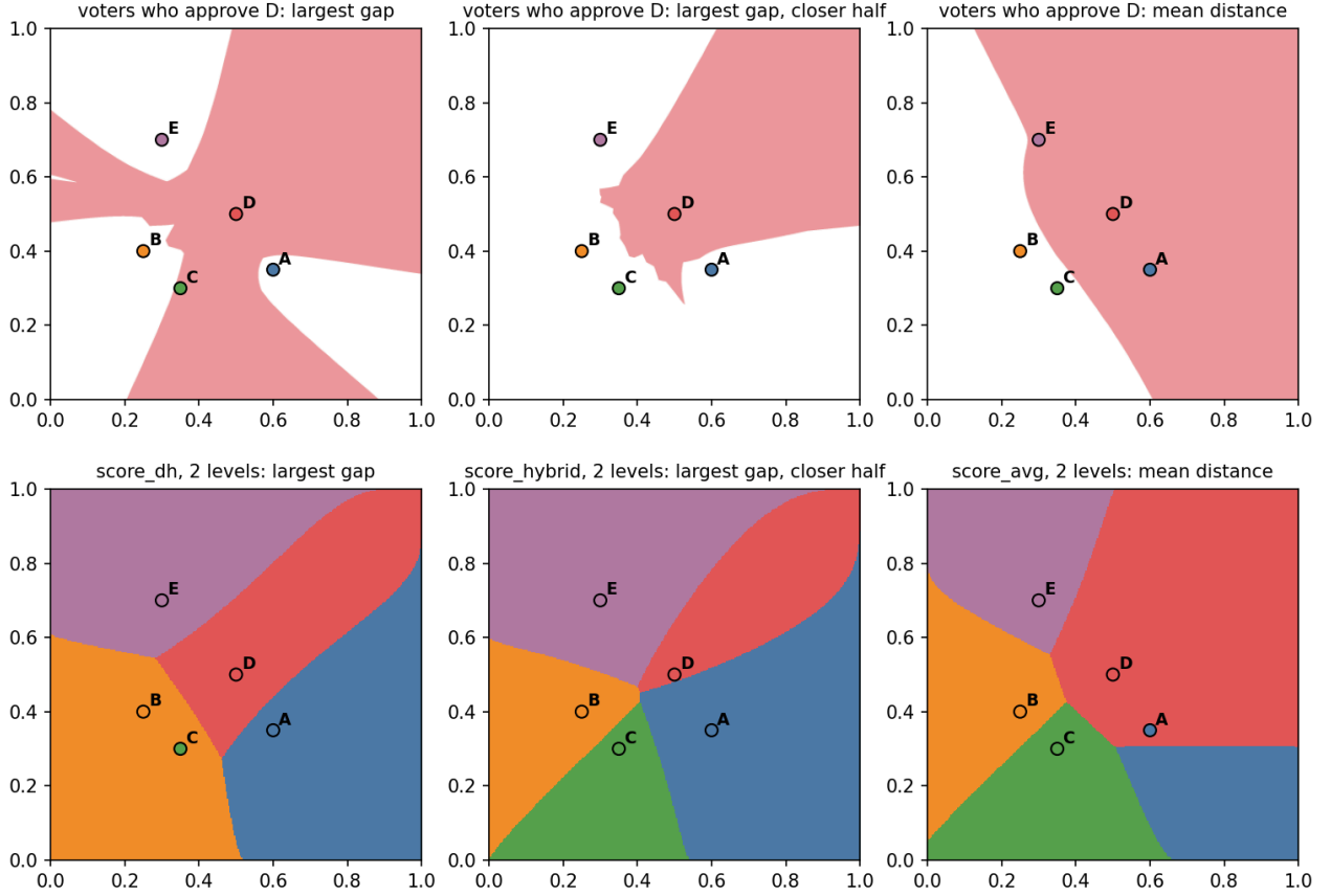
Figure 3: Two levels. Top: the voters who approve D with ScoreDH (above the largest gap), with ScoreHybrid (above the largest gap of the closer half) and with ScoreAvg (closer than the mean distance); the borders are curves. Bottom: the three diagrams (candidates A–E, Beta voters, rms, D = 0.2 ).
