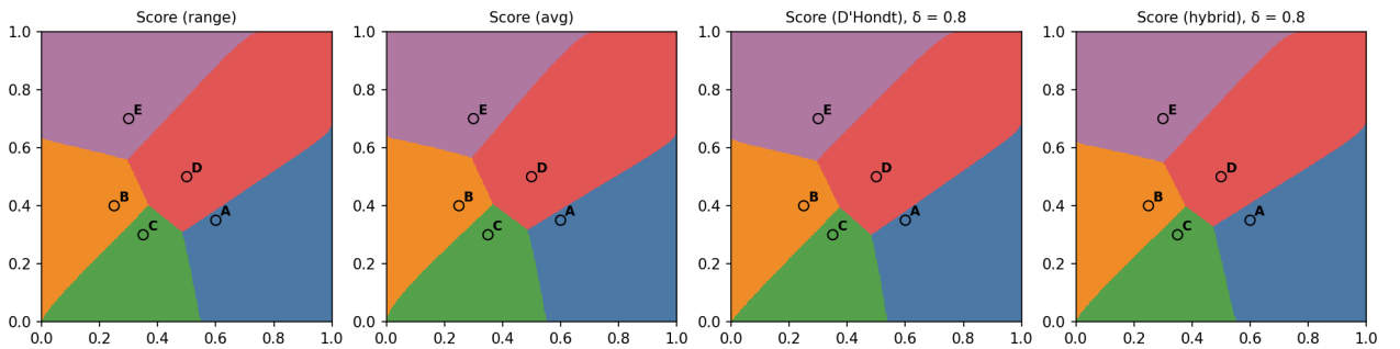
Figure 4: The four rules at the default of six levels, ScoreDH and ScoreHybrid with \delta = 0.8 (candidates A–E, Beta voters, rms, D = 0.2 ).
