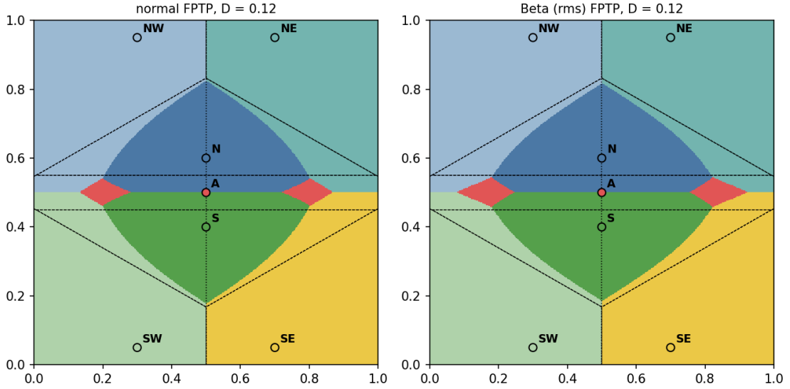
Figure 10: FPTP with normal and Beta voters, D = 0.12 . Dashed: Voronoi borders; dotted: the column x = \frac{1}{2} , where A (red) never wins. A 's region is in two pieces.
