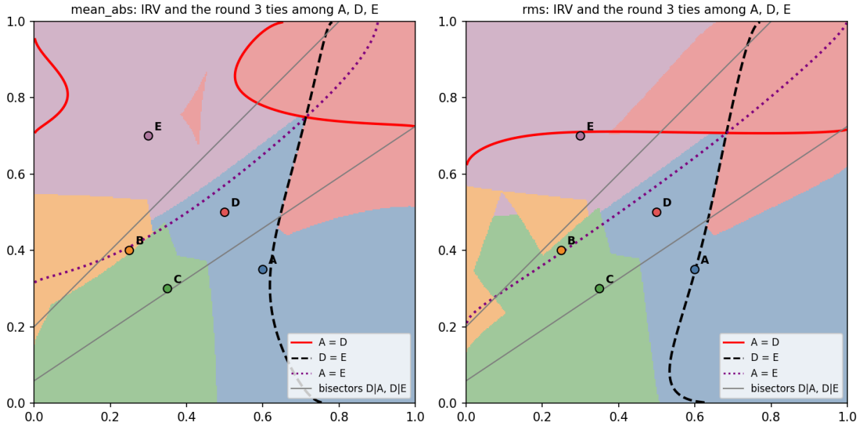
Figure 12: Beta IRV (faded) with the three round 3 tie curves among A, D, E, under mean_abs (left) and rms (right). The red curve s_A = s_D bounds D's region. Gray: the bisectors D|A and D|E.
