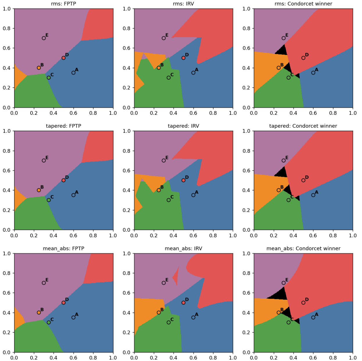
Figure 11: The three spread rules of Section 1.5 on the default candidates, D = 0.3 . Only mean_abs has the round IRV edge. Black: no Condorcet winner.
