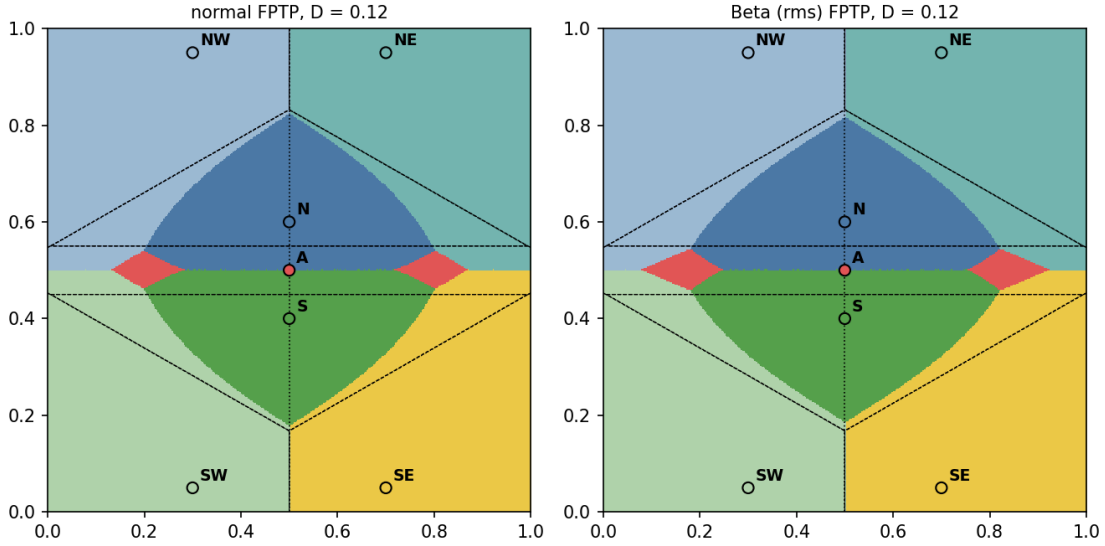
Figure 14: FPTP with normal and Beta voters, D = 0.12 . Dashed: Voronoi borders; dotted: the column x = \frac{1}{2} , where A (red) never wins. A 's region is in two pieces.
