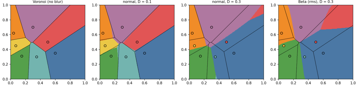
Figure 7: FPTP for seven candidates; dashed: Voronoi borders. From left: no blur (Voronoi), normal voters with D = 0.1 and D = 0.3 , Beta voters (rms) with D = 0.3 .
