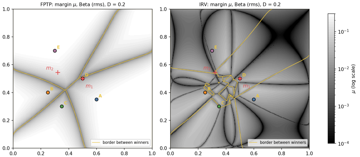
Figure 15: The margin \mu of FPTP (left) and IRV (right) on the grid of G = 320 points per axis (Beta, rms, D = 0.2 ), on a log scale: black is below 10^{-4} . Yellow: the borders between winners, traced as in Section 7.5.2. The crosses mark m_1 (at D) and m_2 .
