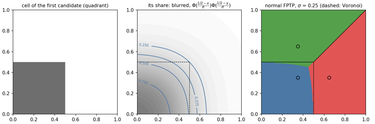
Figure 6: Three candidates whose cells meet at (\frac{1}{2}, \frac{1}{2}) with angles 90^\circ , 135^\circ , 135^\circ (normal voters, \sigma = 0.25 ). Left: the quadrant cell of the lower-left candidate. Middle: its share (Equation 51) with contour lines. Right: FPTP. At the vertex the shares are \frac{1}{4} , \frac{3}{8} , \frac{3}{8} , so the quadrant candidate loses its corner, along a round front.
