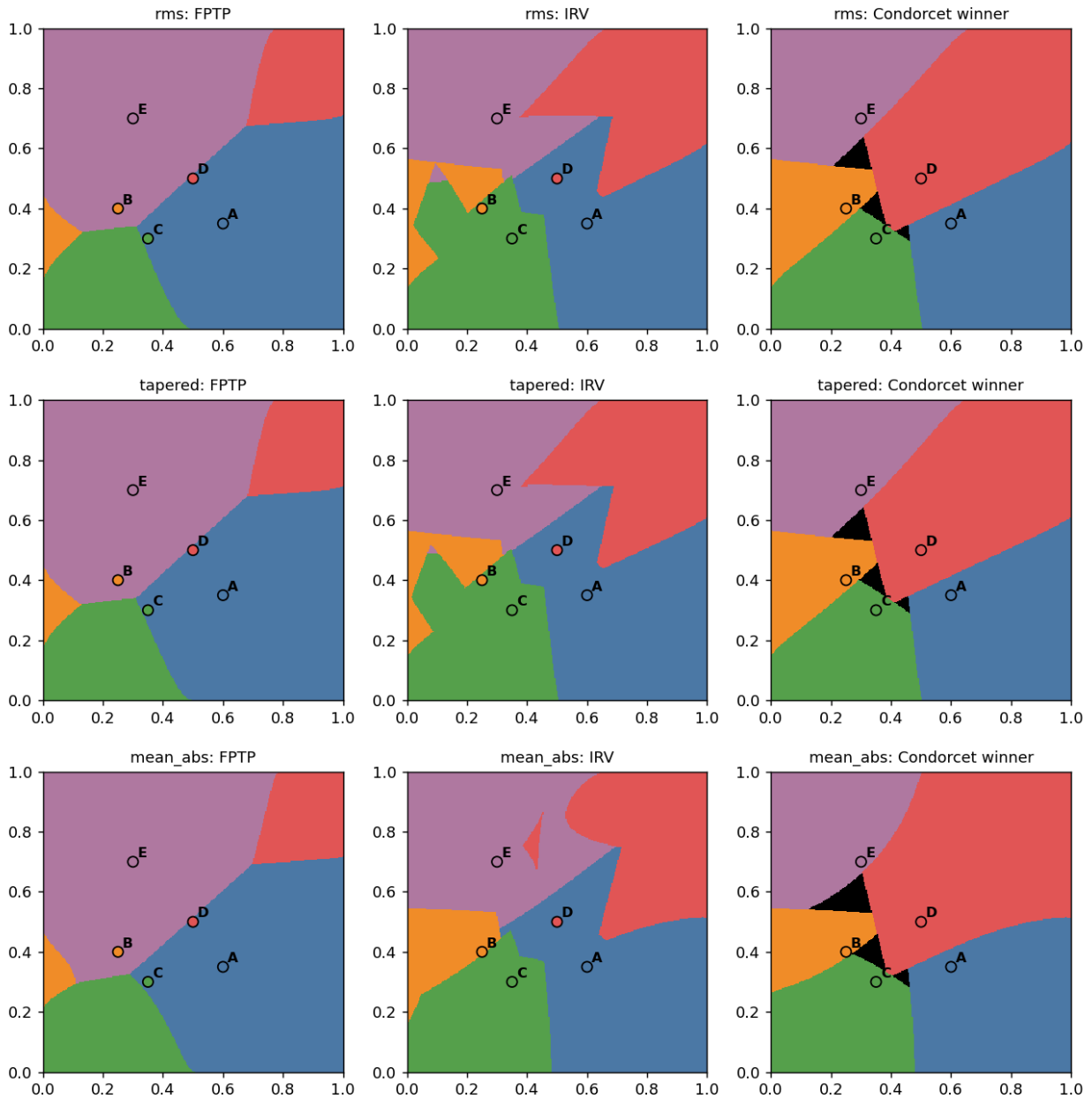
Figure 10: The three spread rules of Section 1.5 on the default candidates, D = 0.3 . Only mean_abs has the round IRV edge. Black: no Condorcet winner.
