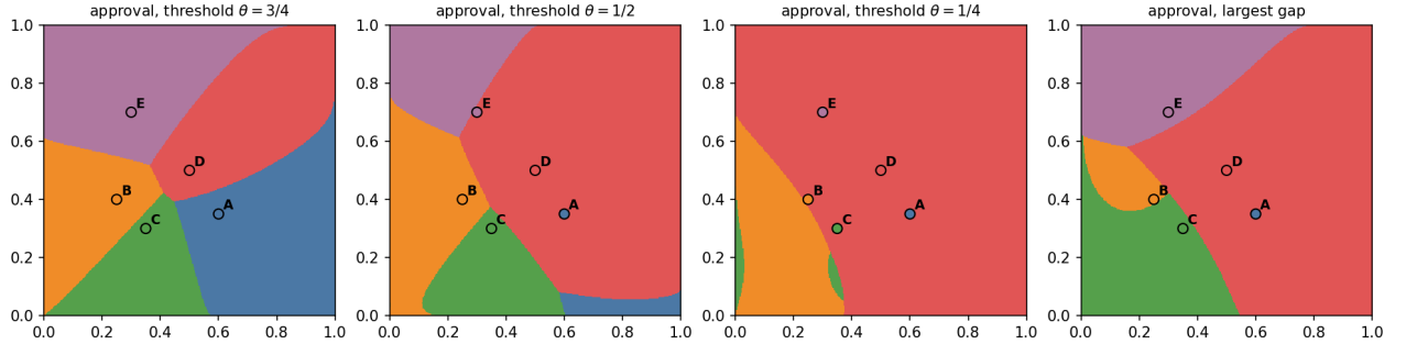
Figure 4: Approval voting at three thresholds and at the largest gap (candidates A–E, Beta voters, rms, D = 0.2 ). The lower the threshold, the more of the square goes to D.
