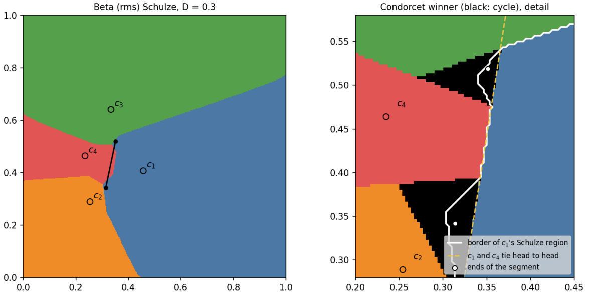
Figure 13: Left: Schulze with Beta voters (rms, D = 0.3 ). c_1 (blue) wins at both ends of the segment, c_4 (red) in between. Right: detail with the Condorcet winner (black: cycles). c_1 's Schulze region, to the right of the white line, reaches across the tie line of c_1 and c_4 (yellow) into two cycle pockets.
