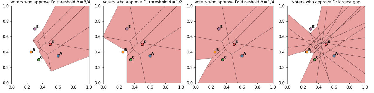
Figure 3: The voters who approve D, as the polygons their share is summed over (candidates A–E). The borders are straight; the thin lines inside are polygon edges, which cancel in D’s share.
