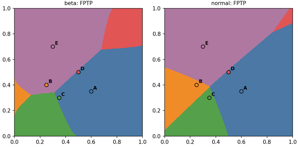
Figure 8: FPTP. With Beta voters the region of B flares out in the last few hundredths before the left wall; with normal voters it widens smoothly.
