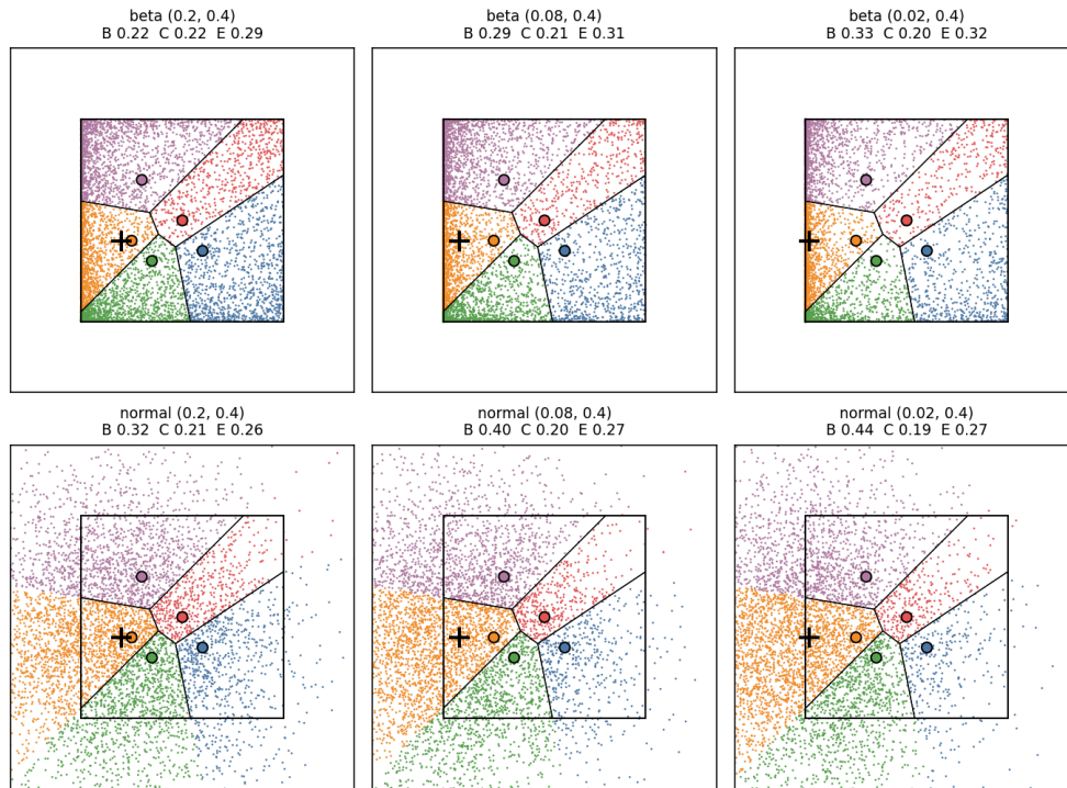
Figure 9: Voters of the pixels (x, 0.4) approaching the left wall, coloured by their first choice (FPTP), with the Voronoi borders; titles: shares of B, C and E.
