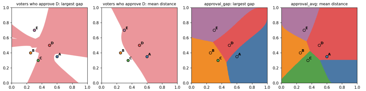
Figure 3: Left: the voters who approve D with GapApproval() and with AvgApproval() ; the borders are curves. Right: the two diagrams (candidates A–E, Beta voters, rms, D = 0.2 ).
