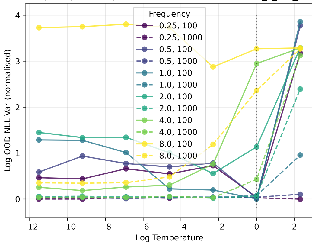
Frequency vs Temperature and OOD NLL Var ood_ll_var_0.1
