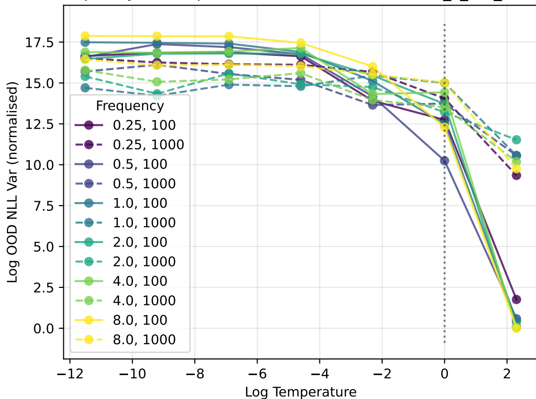
Frequency vs Temperature and OOD NLL Var ood_ll_var_100.0
