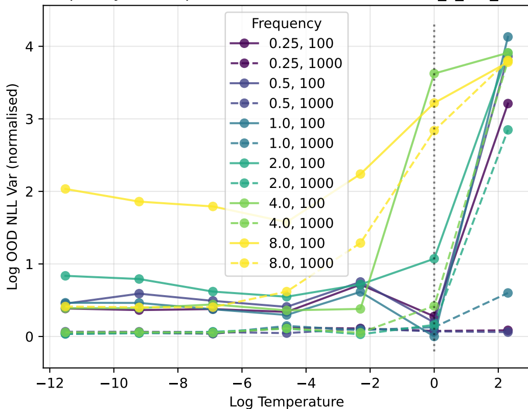
Frequency vs Temperature and OOD NLL Var ood_ll_var_0.01
