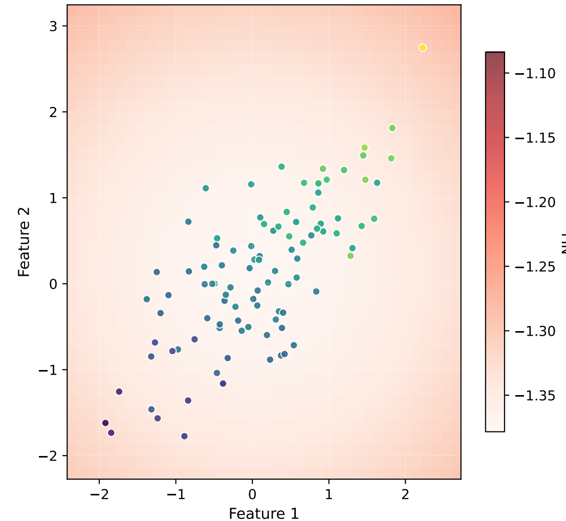
Standard VI Standard ( \lambda=1.0 )
