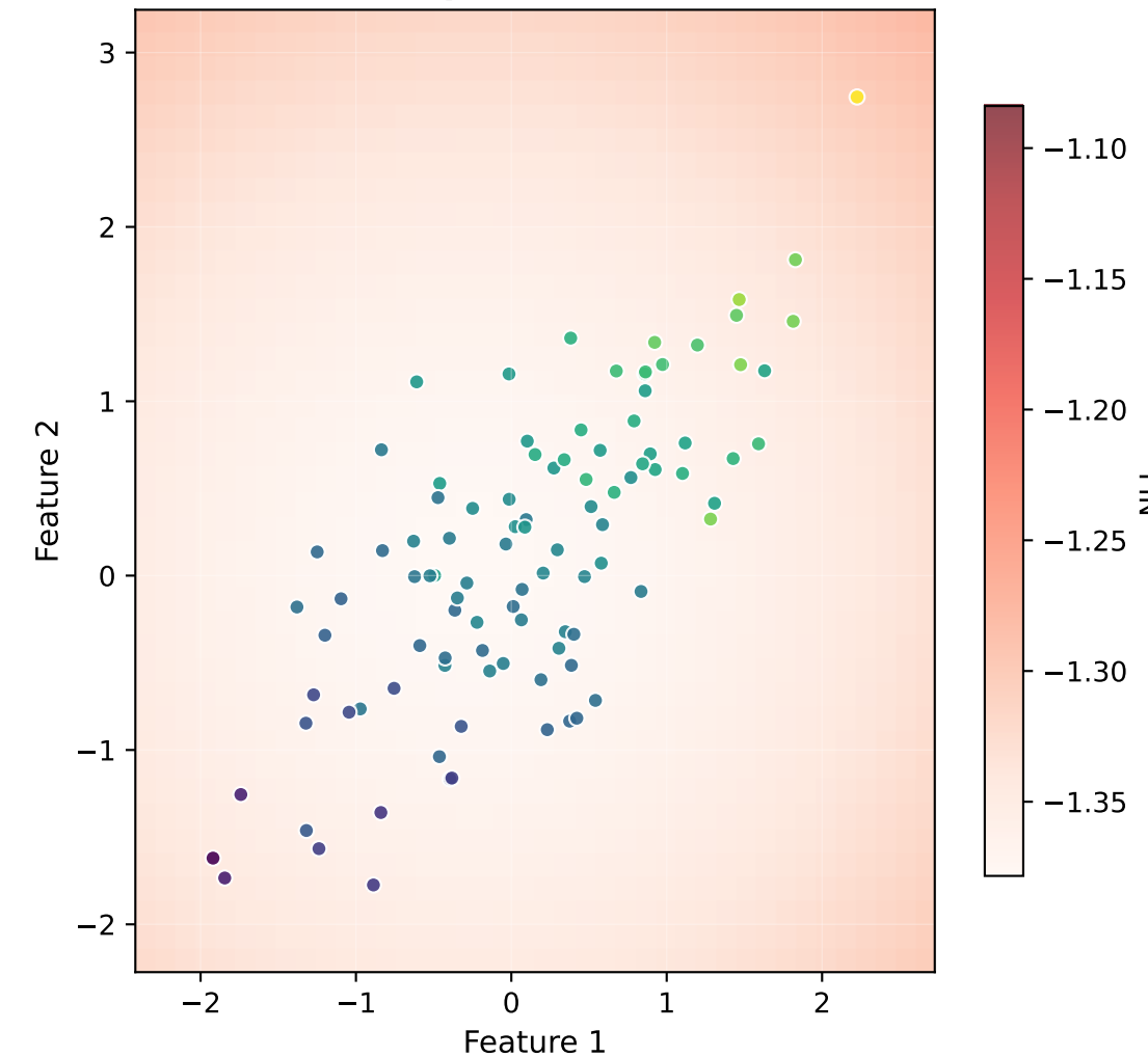
Tempered VI Tempered ( \lambda=0.8 )
