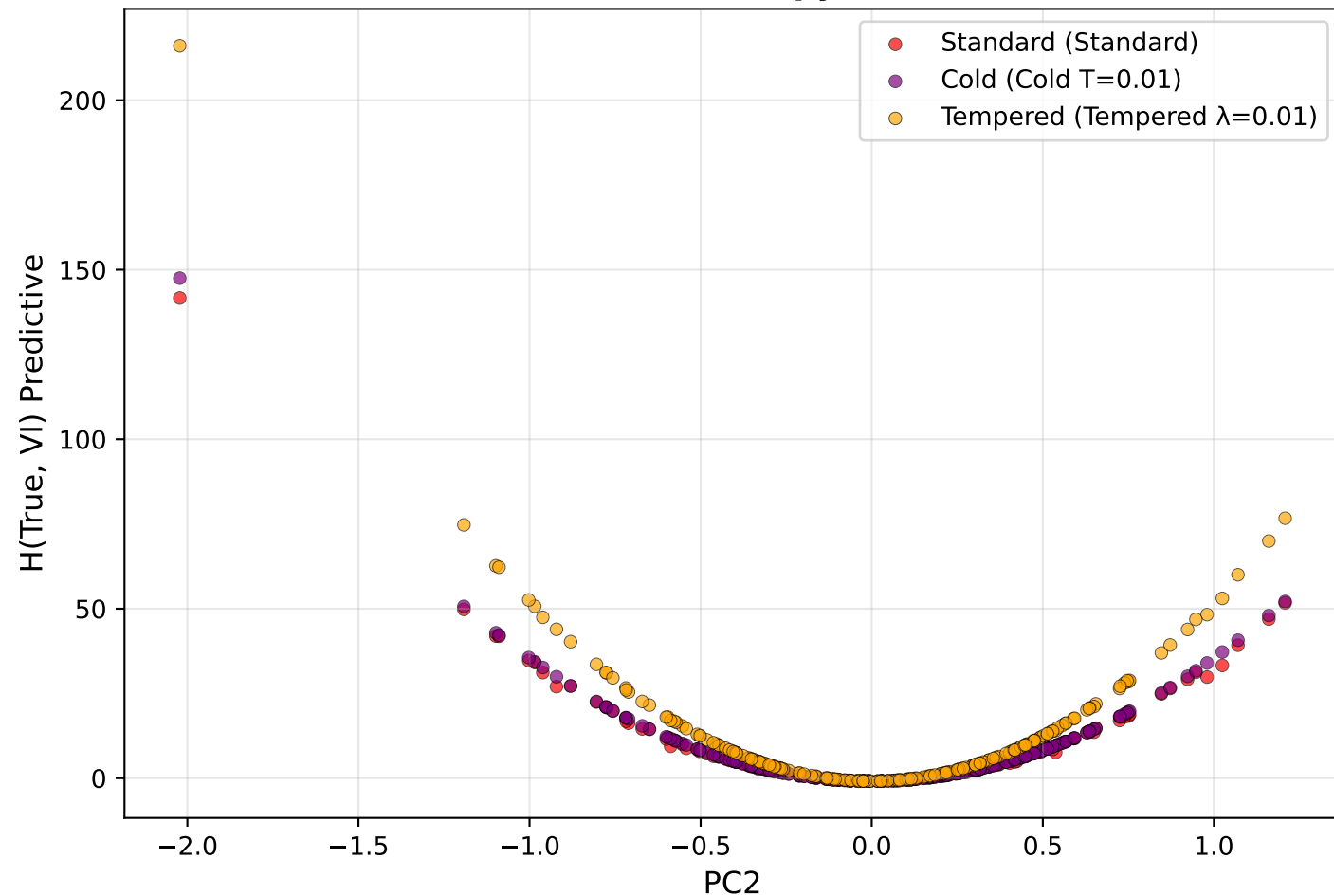
Test Cross Entropy vs PC2
