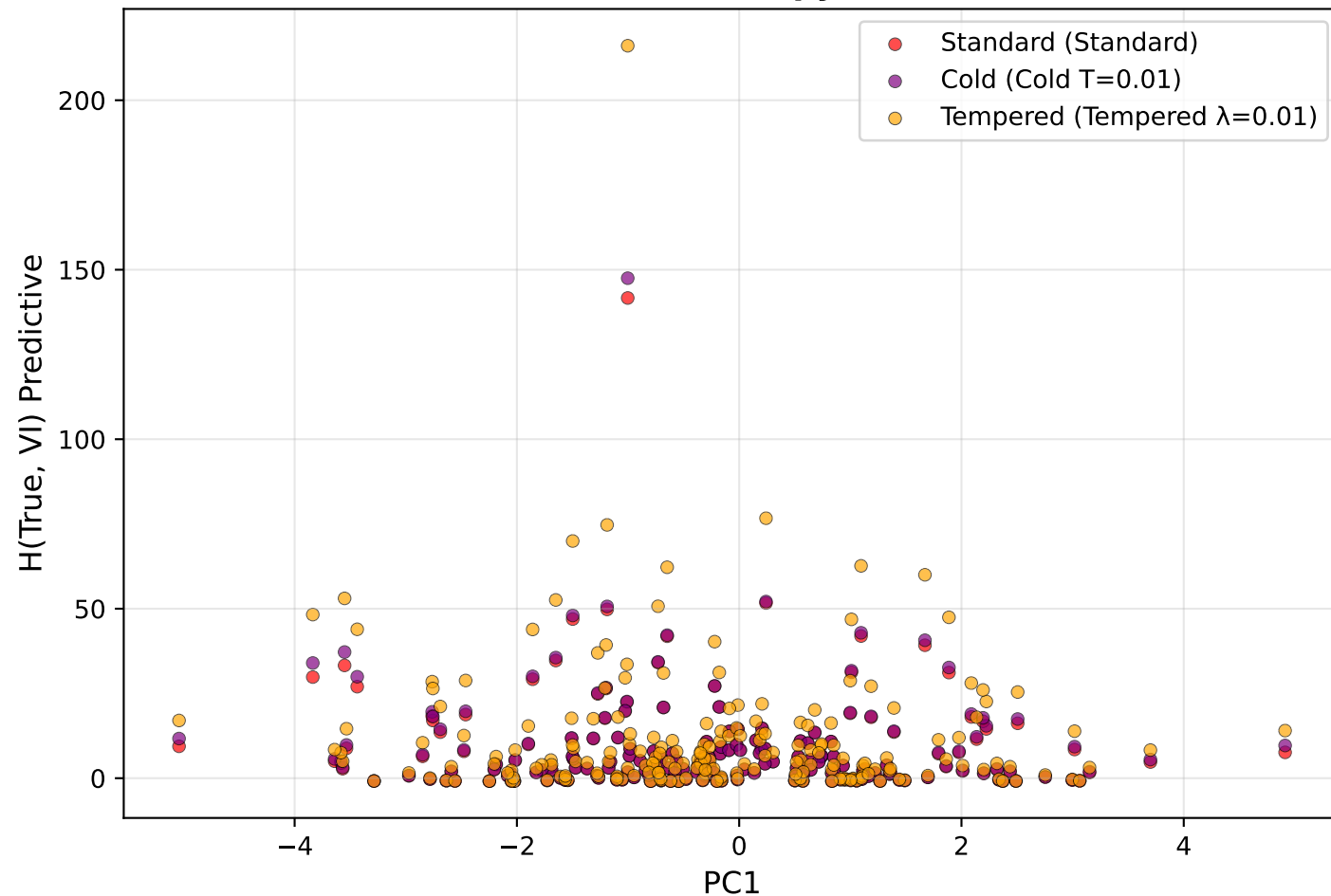
Test Cross Entropy vs PC1
