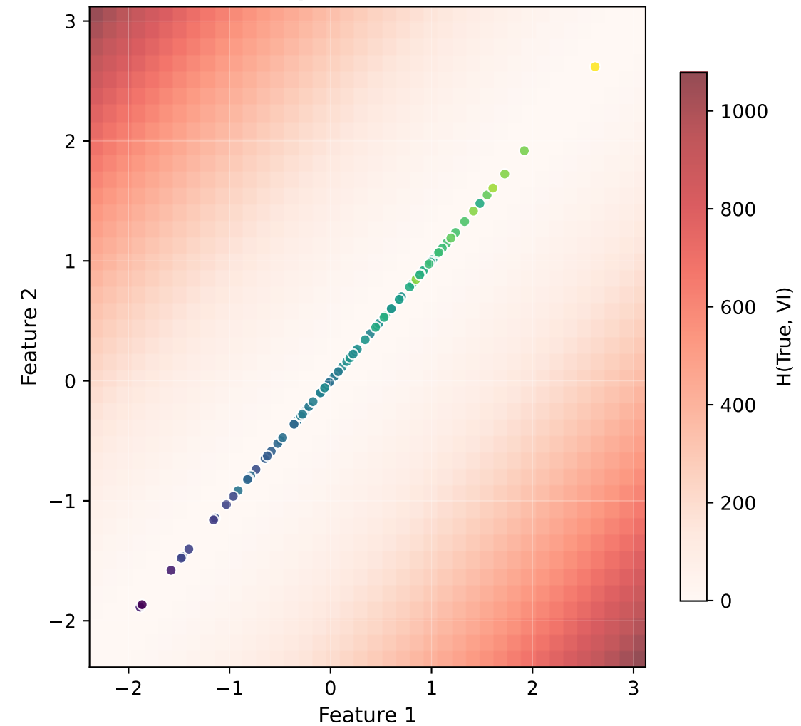
Tempered VI Tempered ( \lambda=0.01 )
