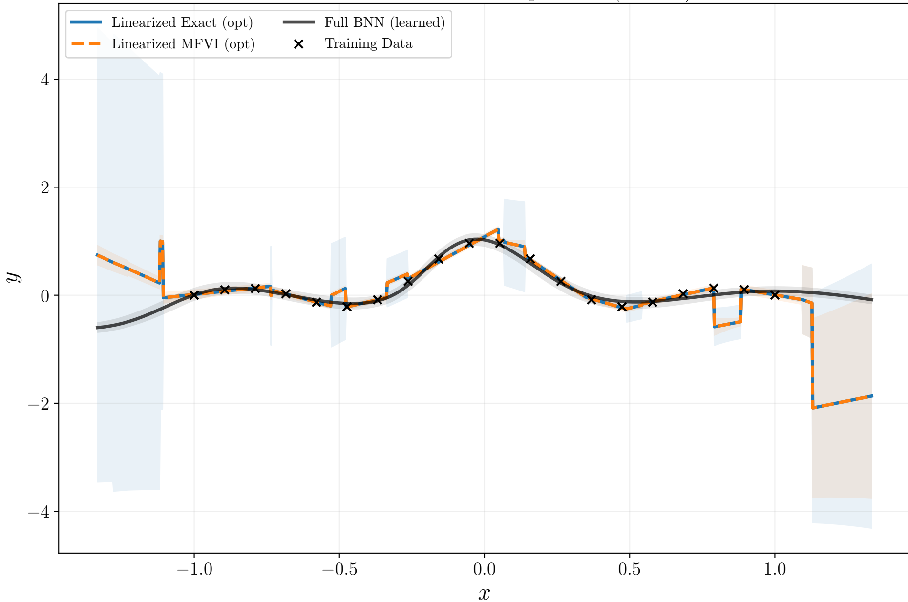
BNN Linearization Comparison (MFVI)
