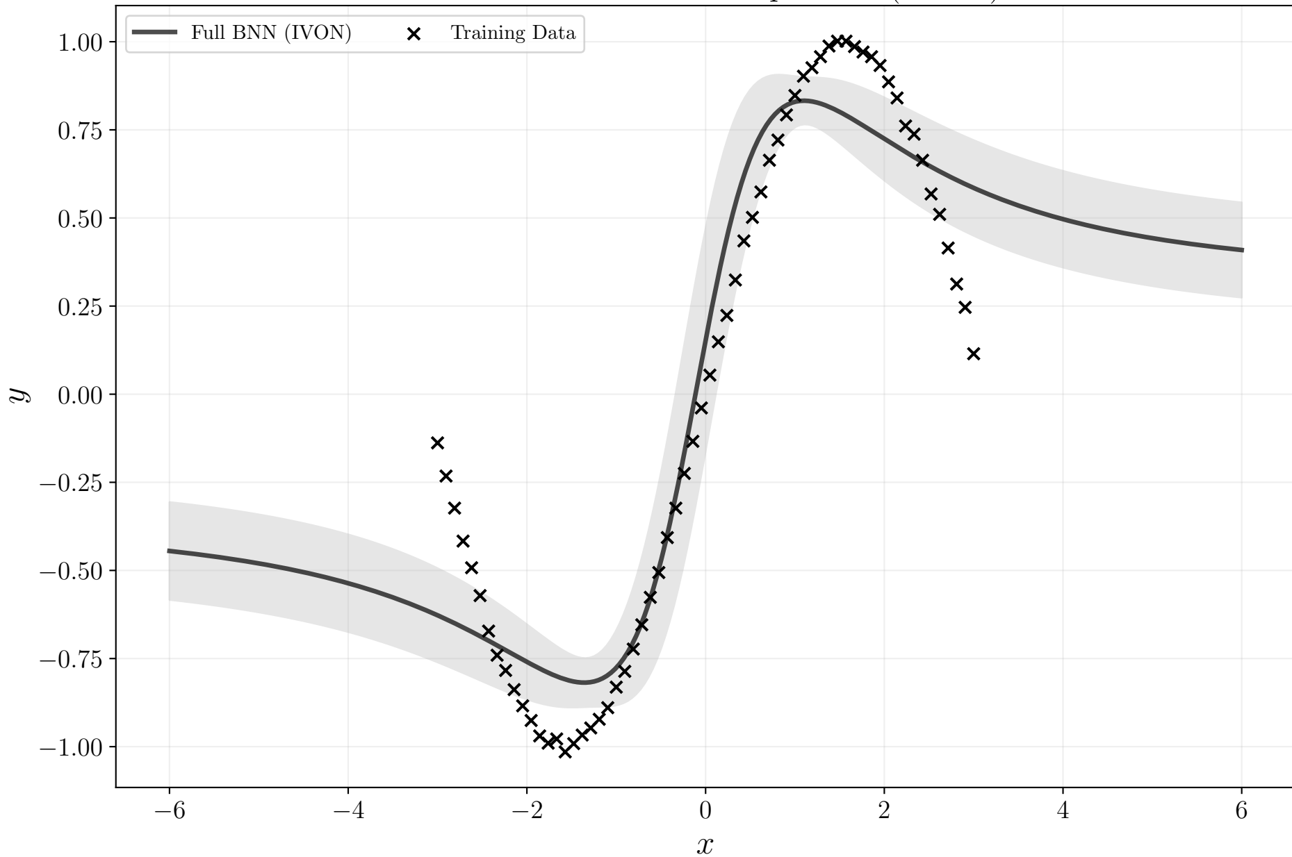
BNN Linearization Comparison (IVON)
