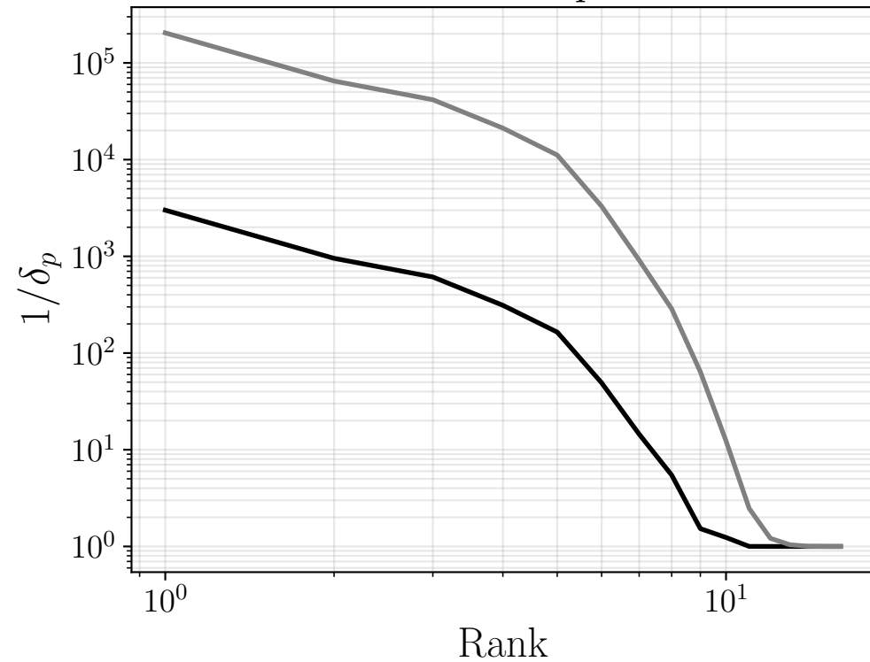
Exact Post. Spectra
